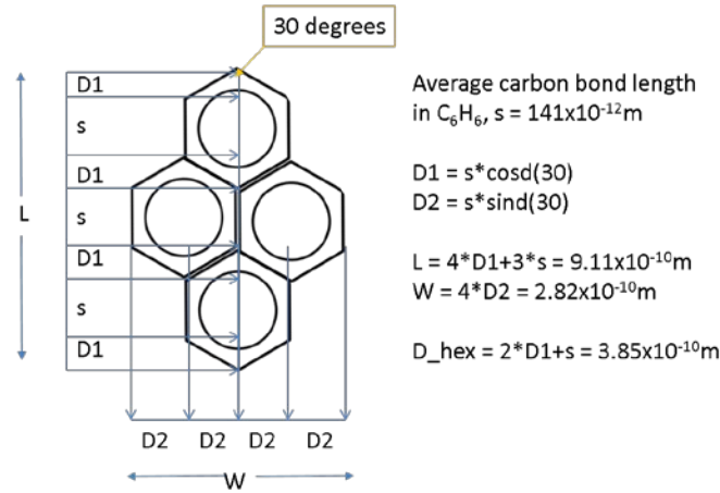
Figure 5: Estimated PBASE dimensions.
