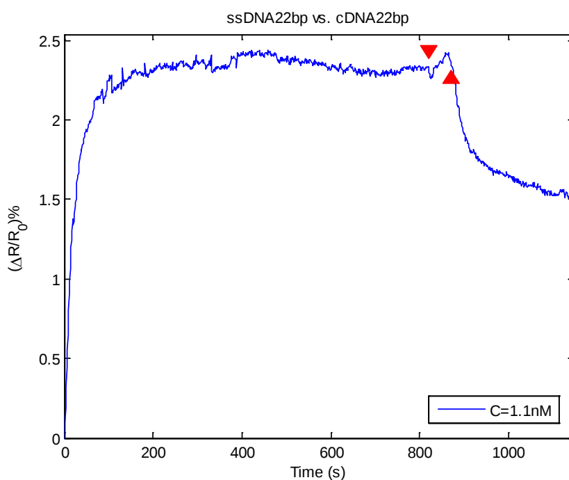
Figure 18: 22bp circuit versus 1.1nM, 22bp target aptamer solution.
