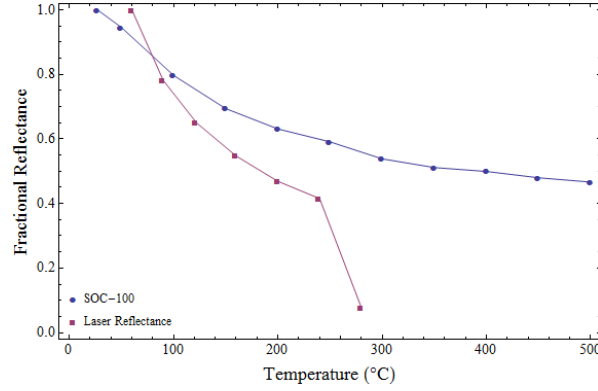
Figure 6.4: Temperature-dependent fractional reflectance of a high-temperature matte black painted sample, with beam incident at 45^\circ and specular reflectance measured with detector at 45^\circ .
