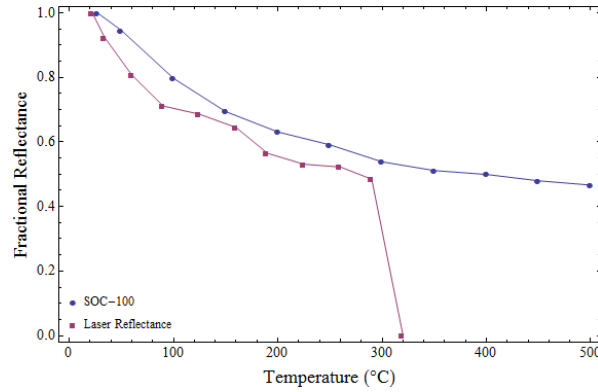
Figure 6.5: Temperature-dependent fractional reflectance of a high-temperature matte black painted sample, with beam normally incident and reflectance measured with detector at 45^\circ .
