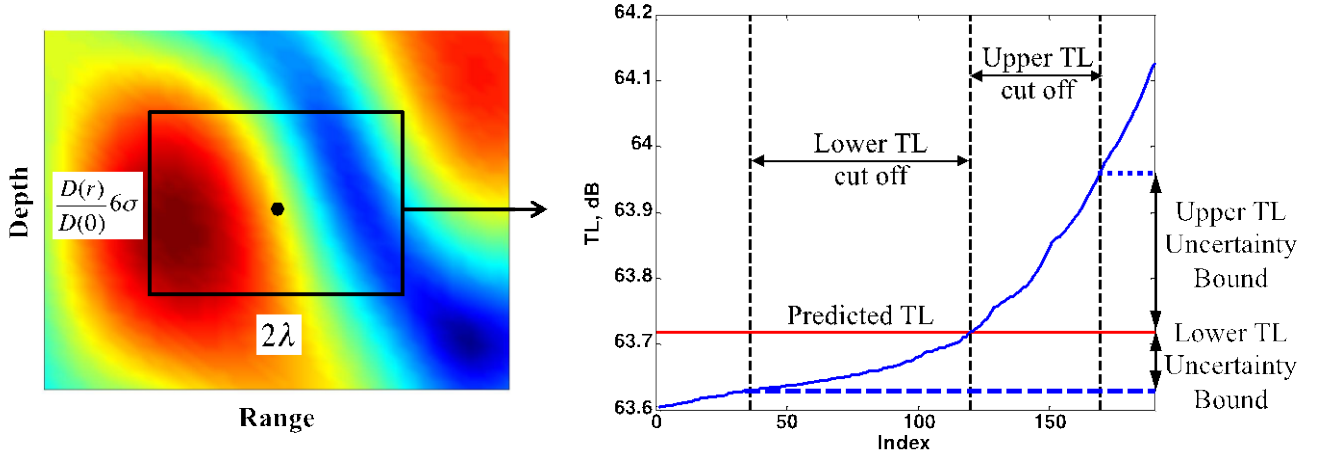
Figure 1. Schematic illustration of the area statistics technique. Here TL values in the range-depth rectangle shown on the left are sorted from lowest (index = 1) to highest TL value. In the example shown there are approximately 190 TL values in the region of interest and the predicted TL value lies at an index of 120. The lower and upper TL cut offs are percentage values used to determine the index values of the upper and lower uncertainty estimates. In this case, these index values are approximately 40 and 170.
