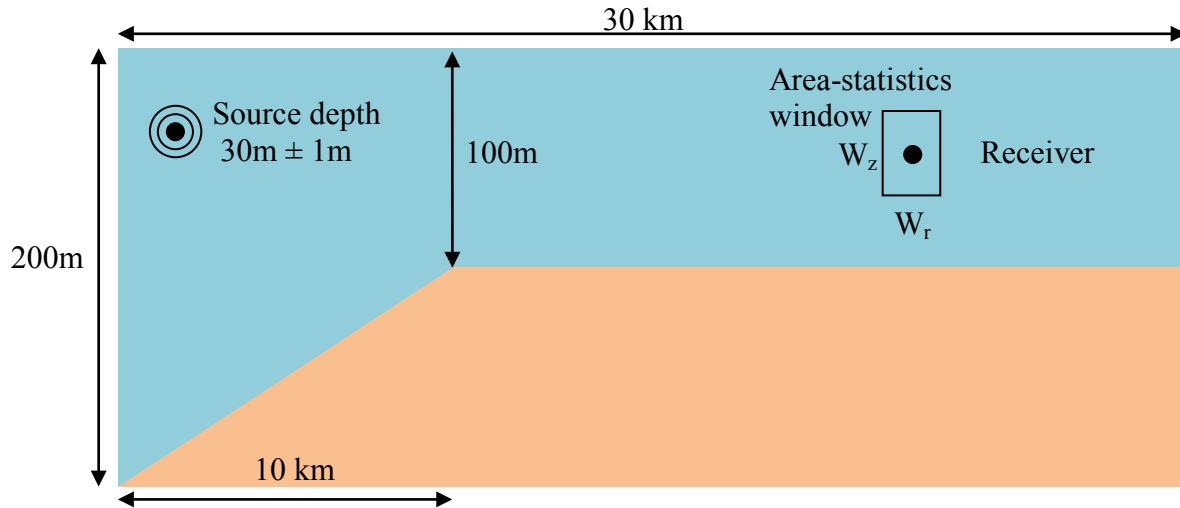
Figure 2. Sample range-dependent environment with uncertain source depth (not to scale). W_r and W_z are the range and depth dimensions, respectively, of the area-statistics window around the receiver.
