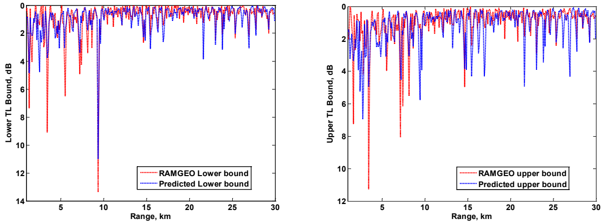
Figure 3. Comparisons of TL uncertainty bounds from area statistics (blue) and direct simulations (red). The left plot is for the lower TL bound and the right plot is for the upper TL bound. In both cases, the agreement is imperfect, but the trend is correct and many of the spikes are matched in location if not in amplitude.
