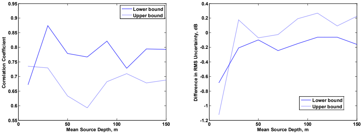
Figure 4. Cross correlation coefficient between the area statistics and direct simulation results for different source depths, and the difference in root-mean-square (RMS) uncertainty between the area statistics and direct simulation results for different source depths. The cross correlations coefficients are near 0.70 and the difference in RMS uncertainties is just a fraction of a dB when the source is away from the ocean surface.
