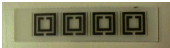
Figure 4 2.5GHz Copper on FR4 meta-atom sample
