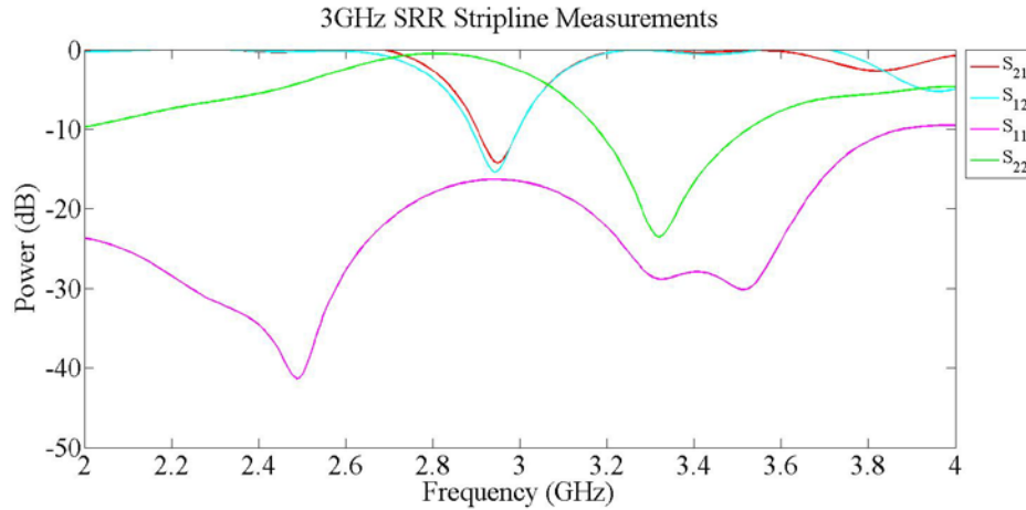
Figure 6 Cu on FR4 stripline measurement with +/-2.5 ns time gating applied by PNA
