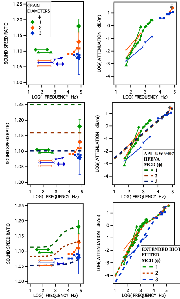
Fig. 2. Measured and inverted sediment sound speeds (top left) and sediment sound attenuation (top right) as a function of frequency at three representative grain sizes 1, 2 and 3 \phi . Comparison with the HFEVA model (middle row). Comparison with the extended Biot model (bottom row).
