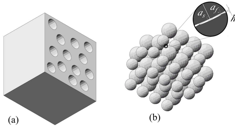
Fig. 1. (a) The skeletal frame in the Biot-Stoll model. (b) The skeletal frame in a granular medium, in which the grain-grain contact is modeled as a solid contact of radius a_s , surrounded by a fluid film of thickness h and radius a_f , as shown in the inset.. [The left panel shows a cube with tubular pores. The right panel shows spherical particles that touch one another. The inset shows a model of the contact region approximated as a solid connection surrounded by a film of fluid.]
