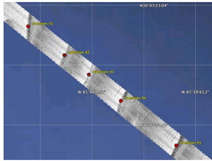
Fig. 3. Map showing the main reverberation measurement track at TREX13, and the detected "transition" zones in which the texture of the sediment appeared to change. [Map of a part of the TREX13 test area showing the initial multibeam survey swath.]
