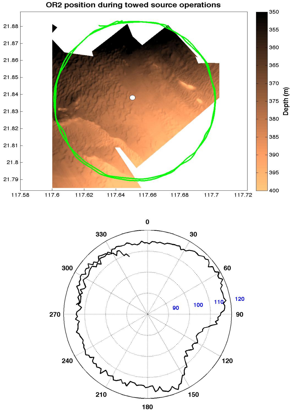
Figure 2. Towed-source track (green circle) around mooring M location (white dot) superimposed on the processed OR5 MBES bathymetric data (top panel), and the corresponding processed MF signal energy level (in dB re 1 \mu \text{Pa}^2 \text{s} ) as a function of bearing angle (bottom panel). The source was towed at a shallow depth ( \sim 10 \text{ m} ).
