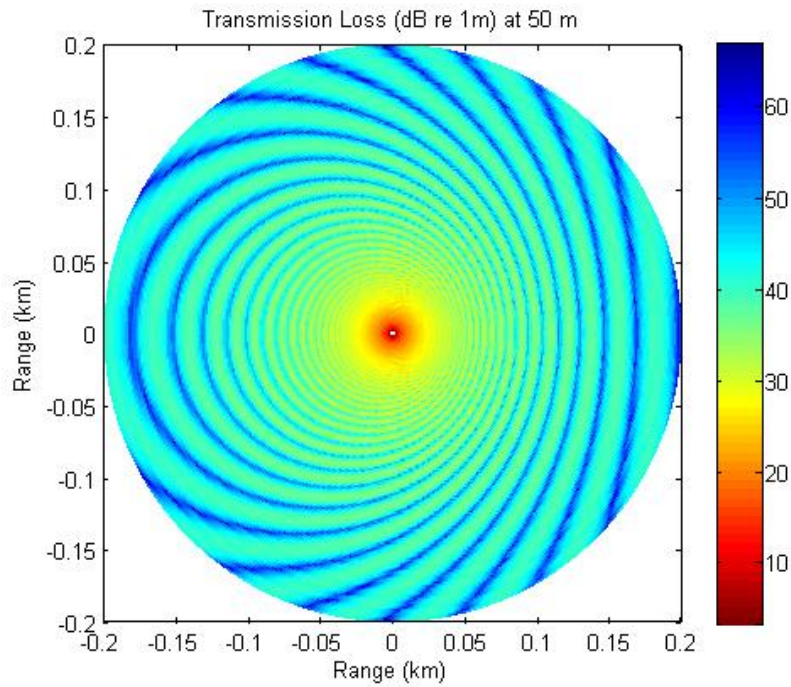
Figure 1: 3-D MMPE test case results for a constant slope, 2-D surface in cylindrical coordinates: TL field along a single radial in the direction of the surface down-slope (upper panel); TL field at a constant depth of 50 m (lower panel).
