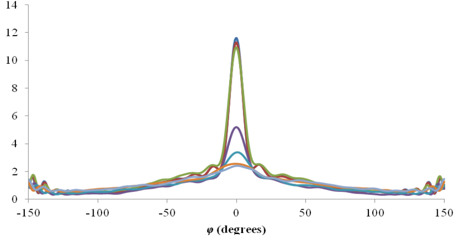
Figure 3. Mean square scattered-field ratio \langle |\psi_s(R, \phi)|^2 \rangle / \langle |\psi_s(R, \phi)|^2 \rangle_{ave} vs. scattering angle \phi for an average scatterer spacing k_{os} = 2.5 . Here scatterers are initially placed in cubical aggregation with a 5-wavelength edge (blue), and the corners and edges of the scattering aggregation are progressively removed by dropping scatterers beyond progressively smaller distances from the center of the aggregation. Results are shown when scatterers are dropped at distances greater than 4\lambda , (red) 3.7\lambda , (green) 3.3\lambda (purple) 3\lambda (light blue), 2.7\lambda (orange) and 2.5\lambda (gray). The amplitude of the peak at \phi = 0 decreases as the corners and edges of the scattering aggregation are removed.
