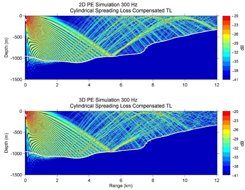
Figure 1. Comparison of 2-D and 3-D PE solutions for underwater sound propagation in the North Mien-Hua Canyon.
