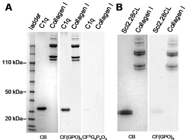
Figure 3. SDS-PAGE of collagen-like proteins stained with CMP. (A) SDS-PAGE loaded with 2 \mu g of complement factor C1q and type I collagen, stained by CB, CF(GPO) 9 , or CF 5 G 9 P 9 O 9 , showing specific visualization of the C1q chains by CF(GPO) 9 hybridization. (B) SDS-PAGE loaded with 2.5 \mu g of type I collagen and streptococcal collagen-like protein Scl2.28CL stained by CF(GPO) 9 , showing almost no staining of the Scl2.28CL band.
