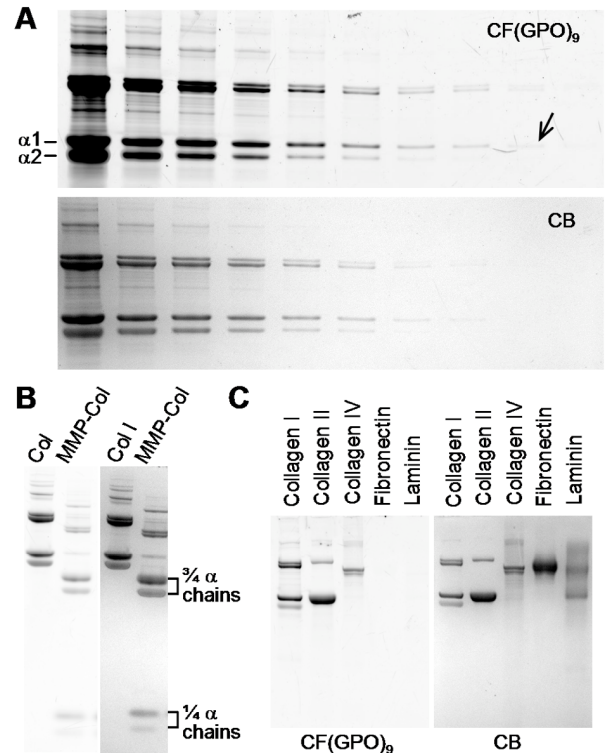
Figure 2-1. Detection of collagen in SDS-PAGE by heat activated fluorescent CMPs. (A) SDS-PAGE loaded with a dilution series of type I collagen, stained and imaged first with CF(GPO) 9 (top panel) followed by coomassie blue (CB) staining (bottom panel). From left to right, each lane was loaded with 4 \mu g, 2 \mu g, 1 \mu g, 500 ng, 250 ng, 125 ng, 62.5 ng, 31.2 ng, 15.6 ng and 7.8 ng of denatured collagen, respectively. The arrow points to the least recognizable band in the image which contains approximately 5 ng of collagen \alpha 1 chains. (B) SDS-PAGE of intact and MMP-1 cleaved type I collagens (3 \mu g in each lane) similarly stained with CF(GPO) 9 and CB. (C) SDS-PAGE loaded with collagen type I, II, IV, fibronectin and laminin (2 \mu g of each protein), and stained with CF(GPO) 9 and CB. (D) Comparative fluorescence levels of the ECM protein bands in SDS-PAGE stained by CF(GPO) 9 (C) or CF S G 9 P 9 O 9 (Supporting Information Figure S3). The measured fluorescence intensities were normalized by collagen I, and the experiment was performed in triplicate ( \pm s.d.). (E) SDS-PAGE of collagen I (0.7 \mu g) and a lysate of HUVECs stained by CF(GPO) 9 and CB showing remarkable specificity of CMP for collagen detection. Images of the CF(GPO) 9 stained gels were recorded using a Typhoon fluorescent imager ( \lambda_{ex} = 488 nm), and CB stained gels were photographed using a Gel Doc EQ system.
