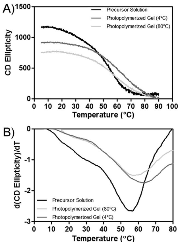
Fig. 1 (A) Circular dichroism melting curves of the PEGDA-CMP precursor solution and PEGDA-CMP gel photopolymerized at 4 °C and 80 °C. (B) First derivatives of corresponding CD melting curves.
