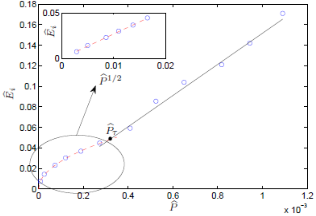
Figure 1: Energy of the inertial range E_i ( \circ ) with respect to the energy flux P in the series of SNOW simulations, with square-root (---) and linear (—) fittings for small and large values of P . Inset: Values ( \circ ) and fitting (---) of E_i with respect to P^{1/2} for lower values of P .
