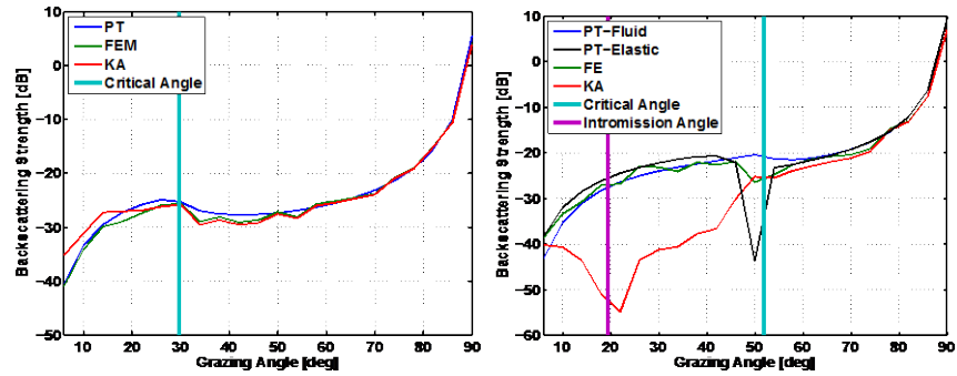
Figure 5: The backscattering strength for a fluid bottom (left) and an elastic bottom (right). Shown are the results from perturbation theory (black), perturbation theory neglecting the shear wave component (blue), finite elements (green) and the Kirchhoff approximation (red). Also shown is the critical angle for the compressional wave and the intramission angle for the shear wave.
