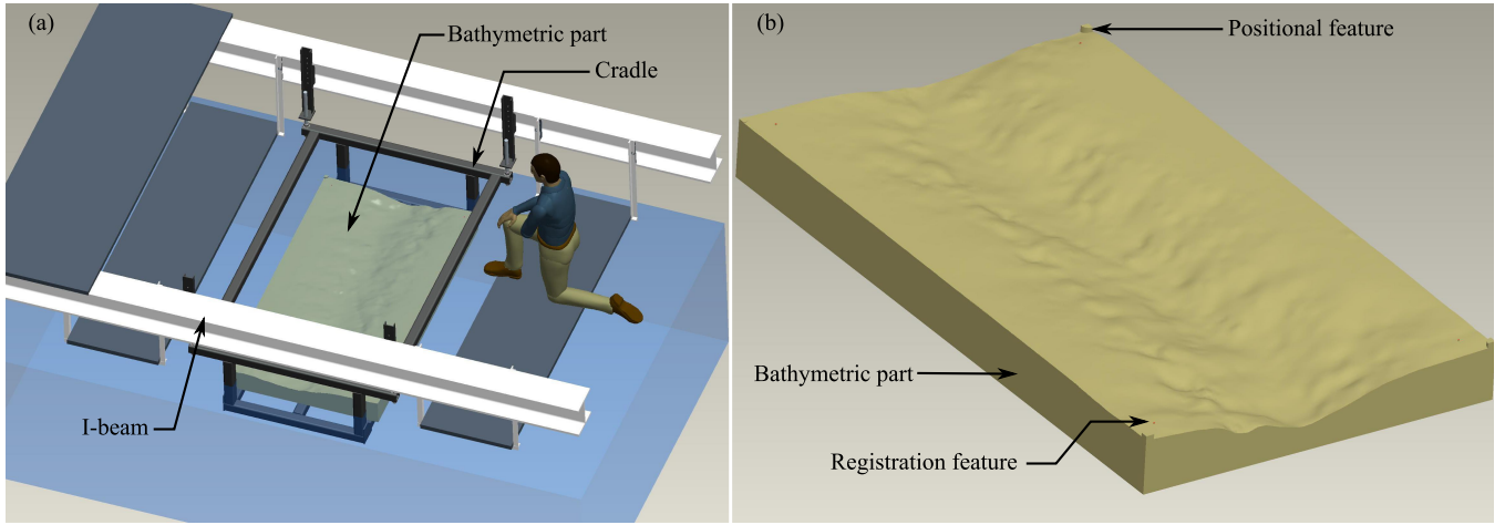
Figure 2: Mechanical design of (a) experimental support structure and (b) scale-model canyon.
