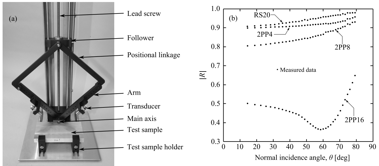
Figure 3: (a) RCM apparatus, (b) magnitude of the reflection coefficient for several candidate polyurethane foams.
