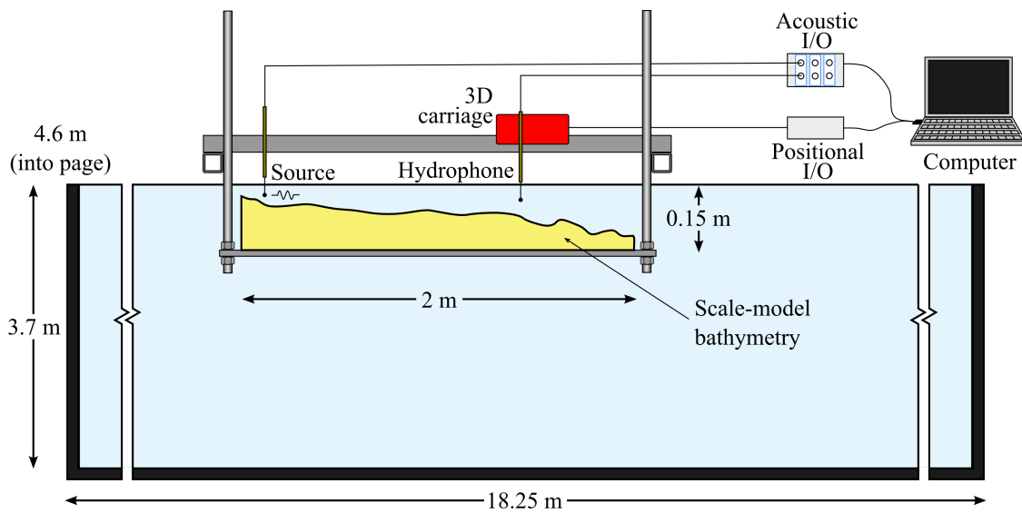
Figure 1: Illustration showing the experimental apparatus.
