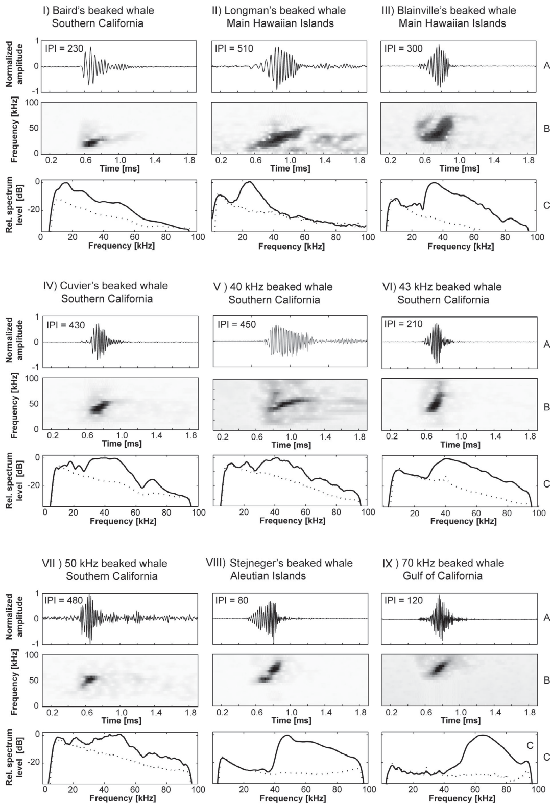
Figure 2. Beaked whale signals known to occur in the Pacific Ocean basin.
