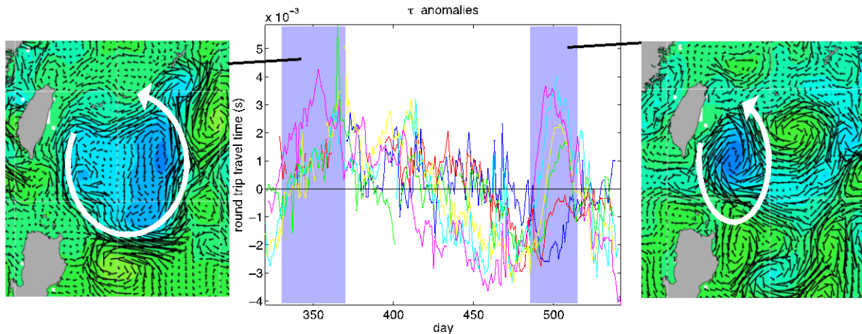
Figure 3. Time series of acoustic-travel-time (means removed) retrieved from the CPIES/PIES in June 2013 via acoustic telemetry. Highlighted periods show times when acoustic-travel times are anomalously long due to a shallower than average thermocline. These times correspond to arrivals of cyclonic eddies (sea surface lows).
