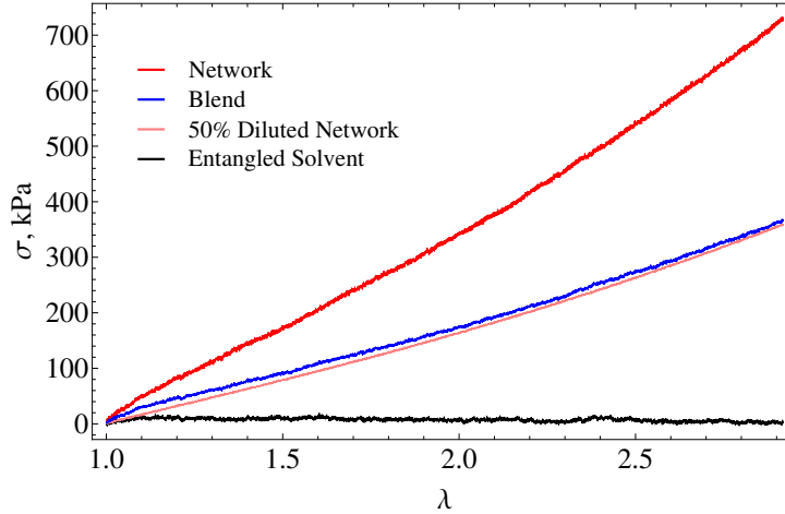
Figure 12. True stress, \sigma , vs. stretch ratio, \lambda for uniaxial tension ( \dot{\lambda} = 5 1/s) using the DSM for N_K^N = 307 , N_K^S = 492 , \beta = 25.3 , and w_{SC} = 0.5 . For the diluted network, \beta^{solution} = 50.6 , N_K^N = 307 .
