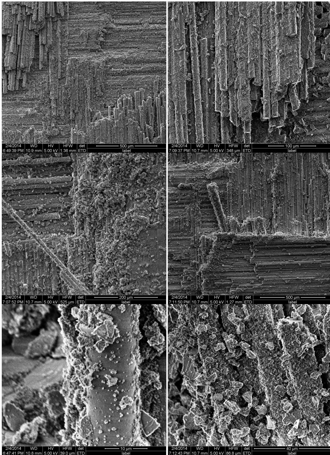
Figure 30. Fracture surface of the DNS specimen tested in creep at 2 MPa at 1100°C in steam, t_f = 96.9 h.
