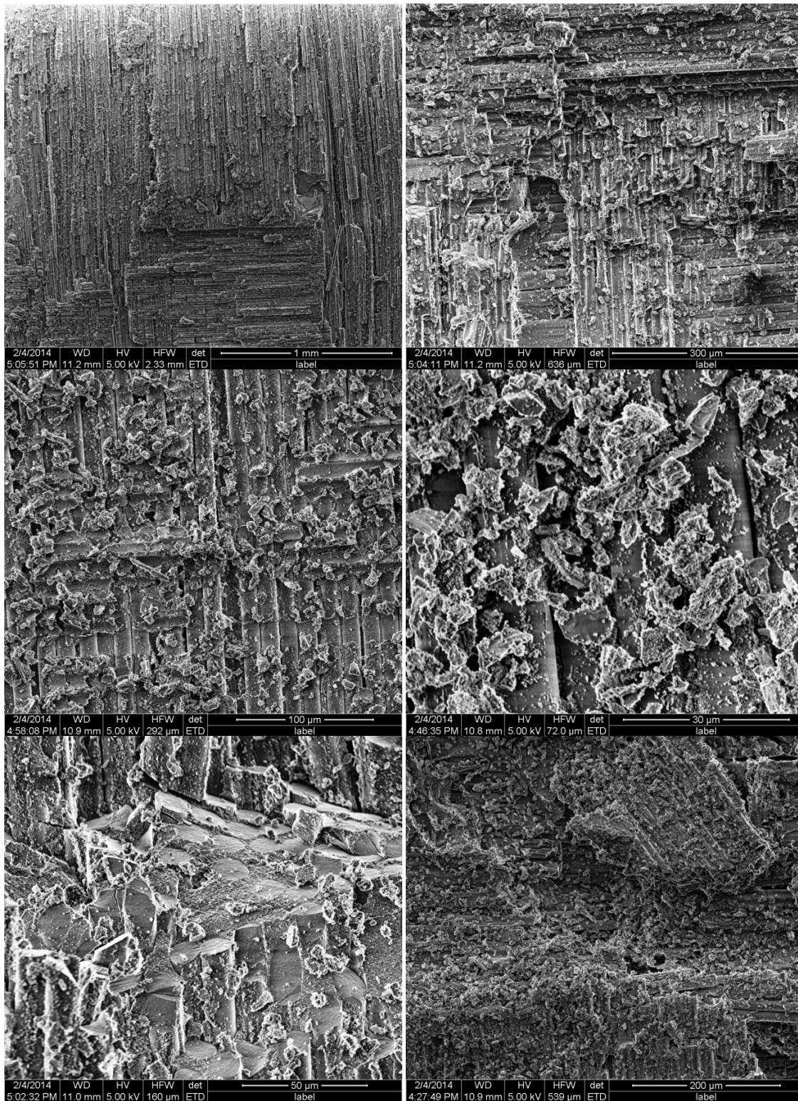
Figure 29. Fracture surface of the DNS specimen tested in creep at 6 MPa at 1100°C in steam, t_f = 22.7 h.
