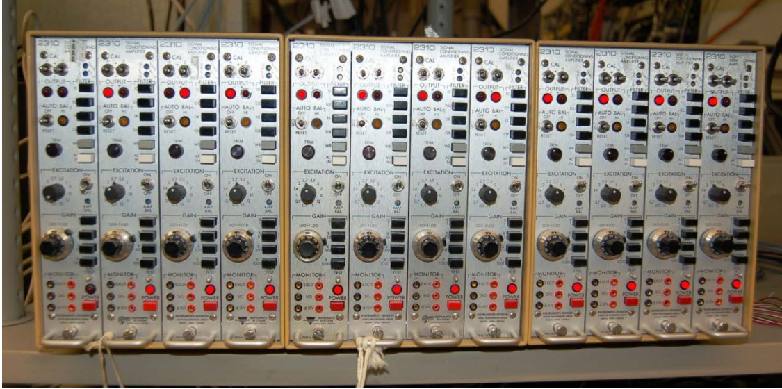
Figure 9. Rack mounted Vishay 2310 strain gage SCAs.
