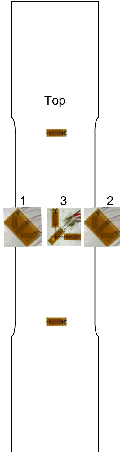
Figure 14. Schematic showing placement of strain gages on a thin-walled tubular specimen. Gage 1 and 2 were 180^\circ apart, gage 3 was 90^\circ with respect to gage 1.
