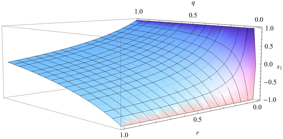
Figure 52. Shows the dependence of the measured s_{1m} values on the extinction ratio of the instrument polarizer. The values of q and r are allowed to vary from 0 to 1. The input Stokes parameters are s_1 = 1 and s_2 = 0 and m'_{01} and m'_{02} are both equal to 0.05.
