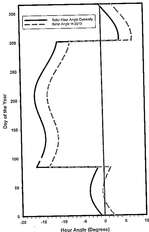
Figure 5. Solar Hour Angle at Greenwich Civil Noon.
