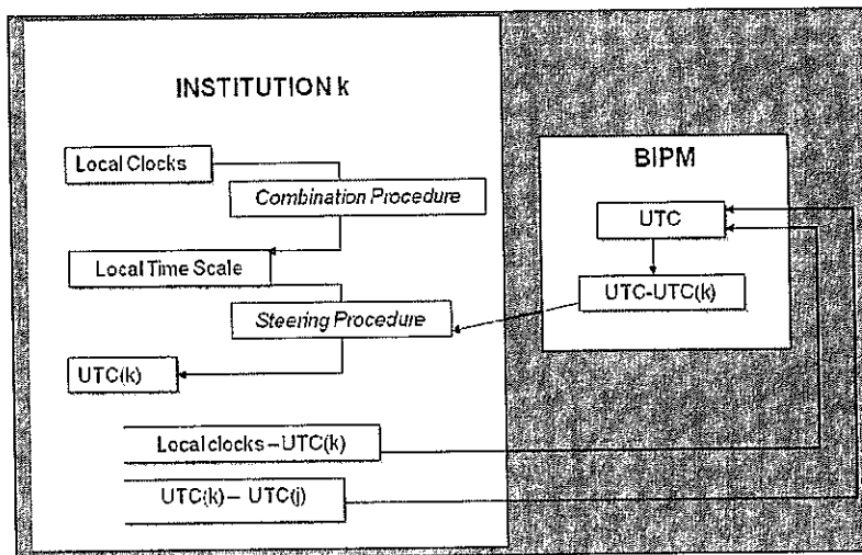
Figure 4. Realization of UTC.
