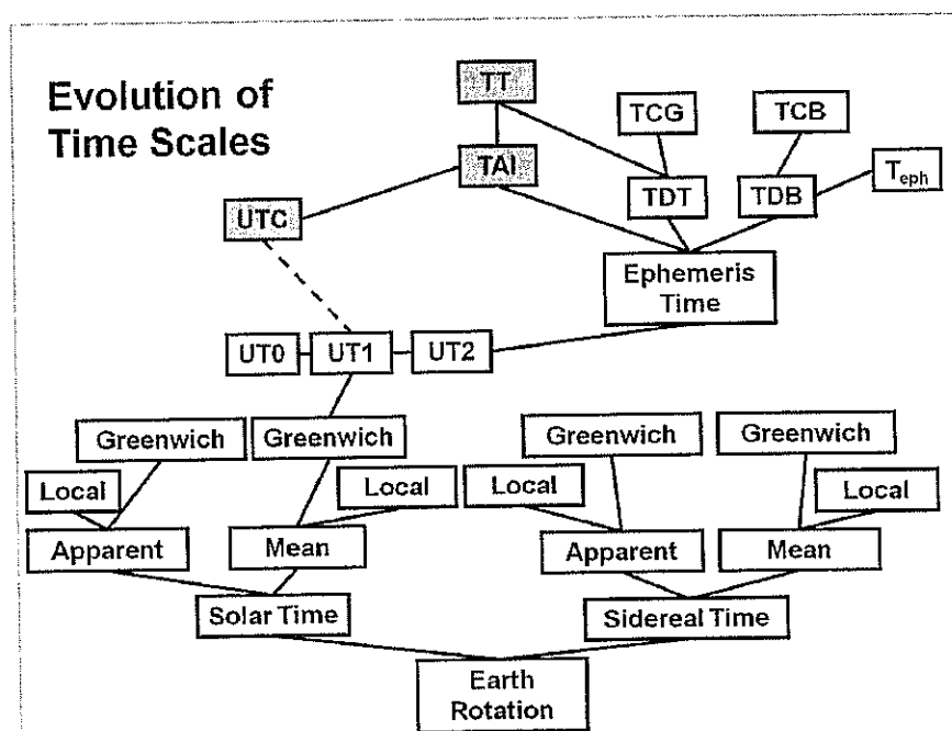
Figure 2. Evolution of Time Scales.
