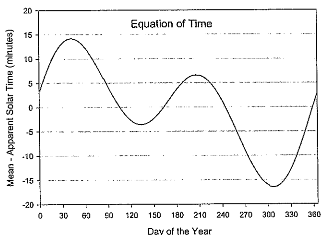
Figure 1. Equation of Time.
