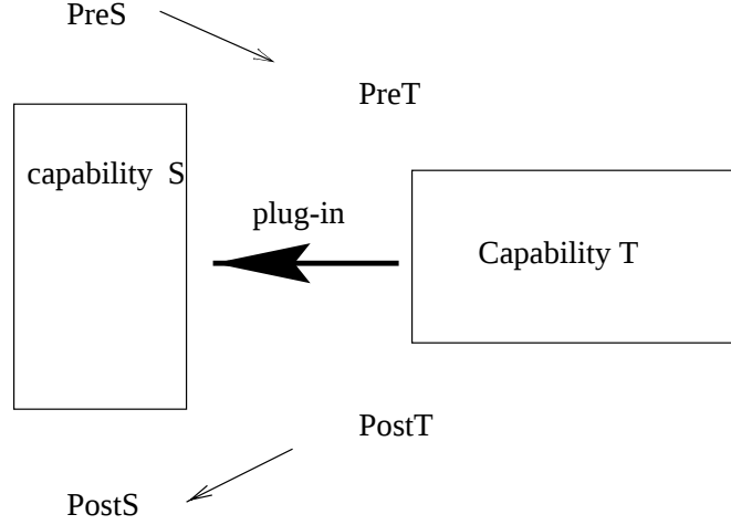
Figure 3: Plug-In Match of Specifications: T plugs into S .
