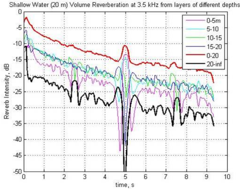
Figure 2. Normalized monostatic reverberation intensity from scattering layers located at different depths (0-5, 5-10, 10-15, and 15-20 m) in water column (having 20m depth) and in a sandy sediment half-space (20-inf) bottom. “Normalized” means “per unit volume scattering strength”, i.e. reverberation intensity calculated assuming the same volume scattering strengths for all scattering mechanisms. This allows then a fast estimation of potential contributions of different mechanisms of scattering with arbitrary strengths and locations.
