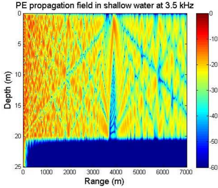
Figure 1. PE propagation field's magnitude in a very shallow water (having 20m depth) at 3.5 kHz, for a source located at a distance 1m above a sandy half-space (non-stratified), calculated using a PE code [13]. These calculations are used then as inputs (through a double propagator) to a simple model of monostatic volume reverberation illustrated in Figure 2.
