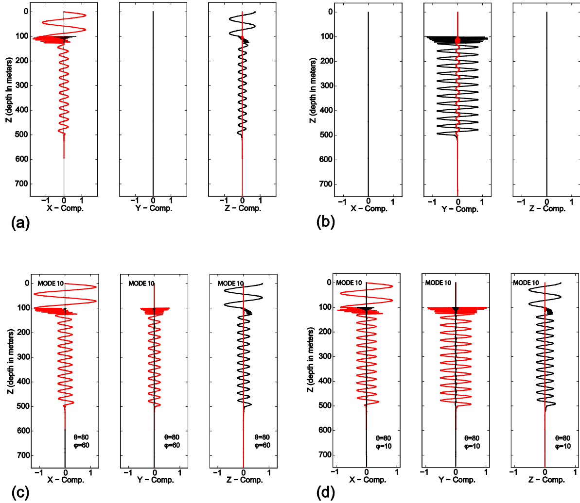
Figure 2. Modes of a seismo-acoustic wave in a shallow water model with a vertical anisotropic symmetry axis (Figures 2a and 2b) for which the horizontally polarized shear waves (SH) propagate completely independently of the compressional and vertically polarized shear waves (P-SV), and for a model for which the anisotropic symmetry axis is tilted away from the vertical, and P-SV and SH are strongly coupled together. Excitation of the SH cannot be avoided for an anisotropic medium with a tilted symmetry axis (Figures 2c and 2d).
