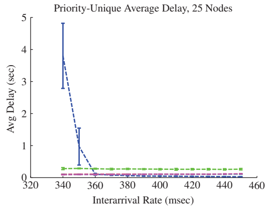
Figure A.158: N25 Packet Delay
