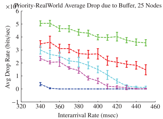
Figure A.291: N25 Buffer Dropped Data
