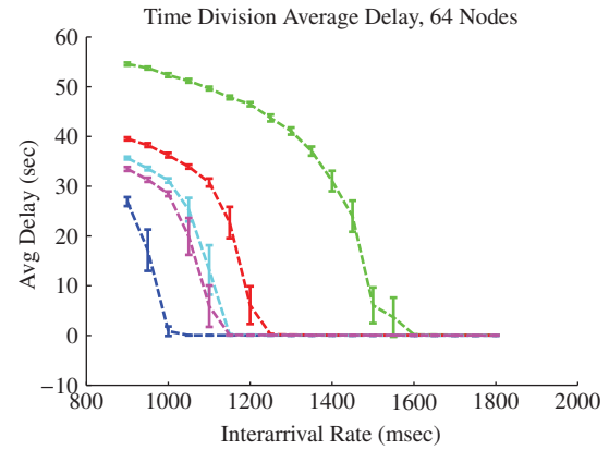
Figure A.128: N64 Packet Delay
