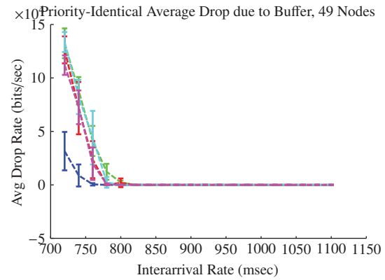
Figure A.211: N49 Buffer Dropped Data
