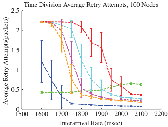
Figure A.137: N100 Retry Attempts
