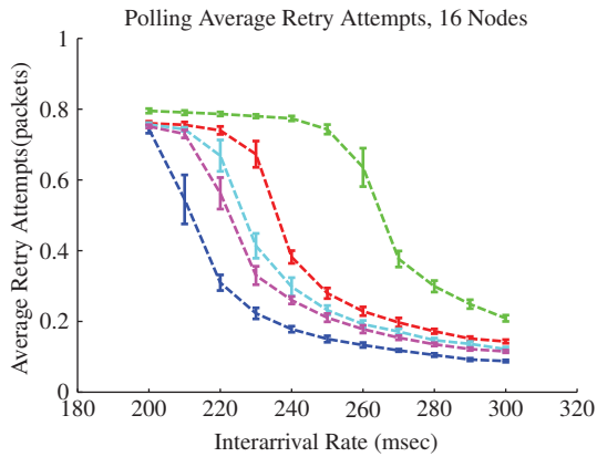
Figure A.62: N16 Retry Attempts
