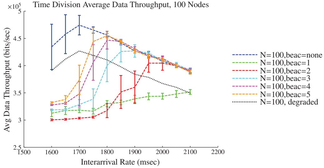
Figure A.134: N100 Data Throughput
