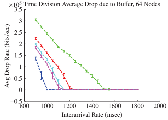
Figure A.126: N64 Buffer Dropped Data
