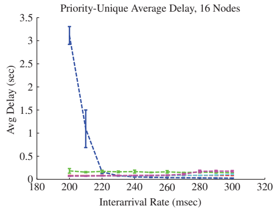
Figure A.153: N16 Packet Delay
