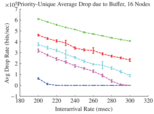
Figure A.151: N16 Buffer Dropped Data
