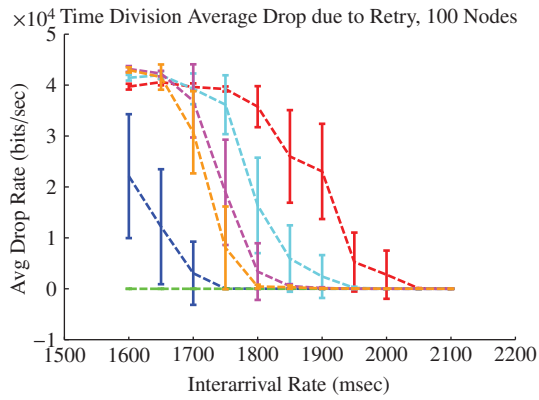
Figure A.135: N100 Retry Dropped Data
