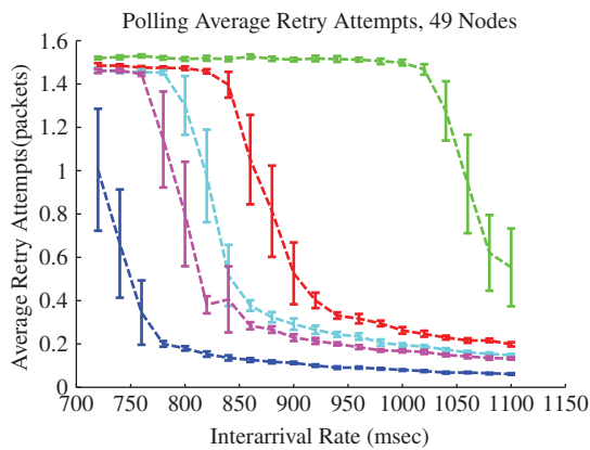
Figure A.77: N49 Retry Attempts
