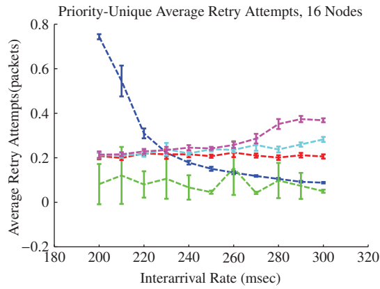
Figure A.152: N16 Retry Attempts
