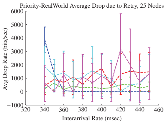
Figure A.290: N25 Retry Dropped Data
