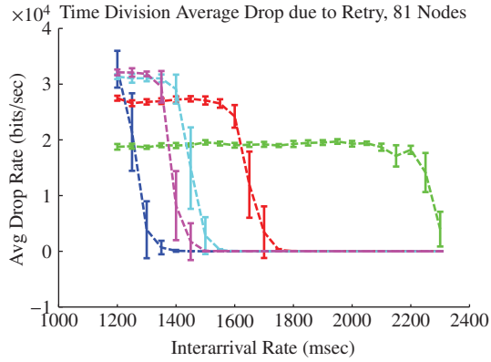
Figure A.130: N81 Retry Dropped Data
