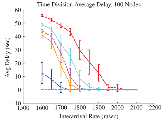
Figure A.138: N100 Packet Delay
