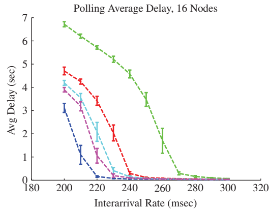
Figure A.63: N16 Packet Delay
