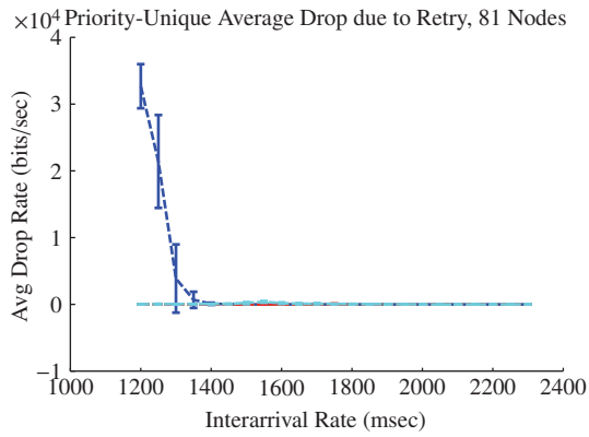
Figure A.175: N81 Retry Dropped Data
