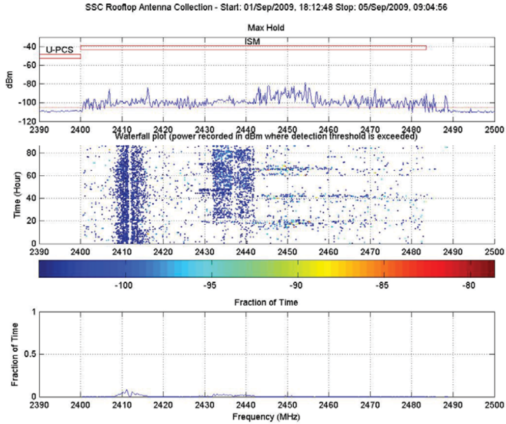
Figure 2.2: 2.4GHz to 2.5GHz usage Vienna, VA [32]
