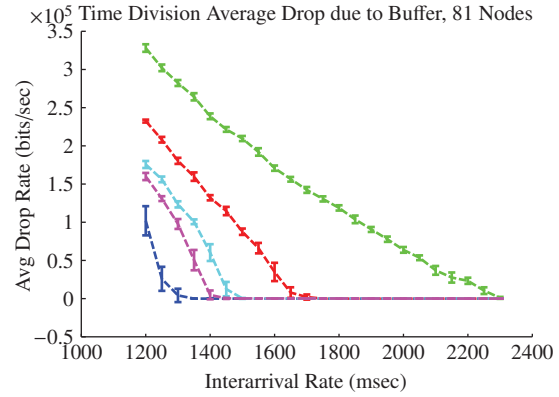
Figure A.131: N81 Buffer Dropped Data
