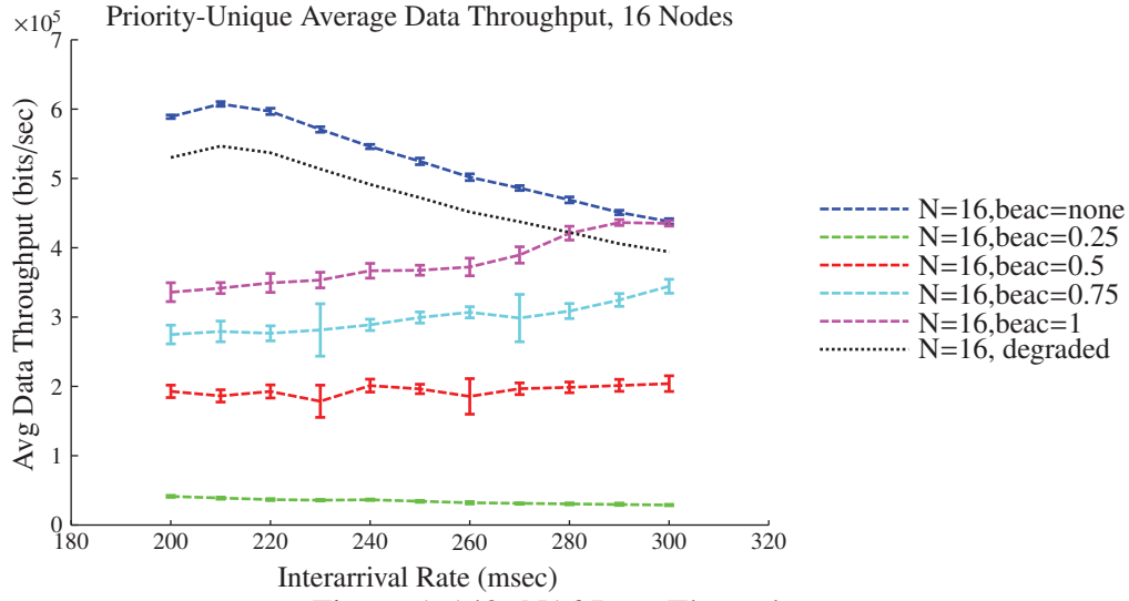
Figure A.149: N16 Data Throughput
