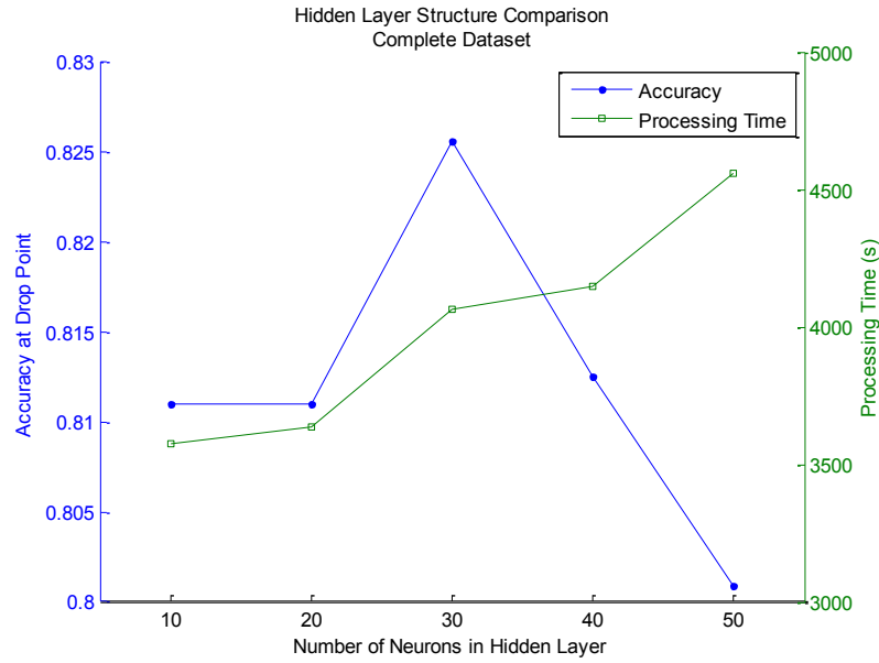
Figure 4.10: Hidden Layer Structure Comparison - Complete Dataset
