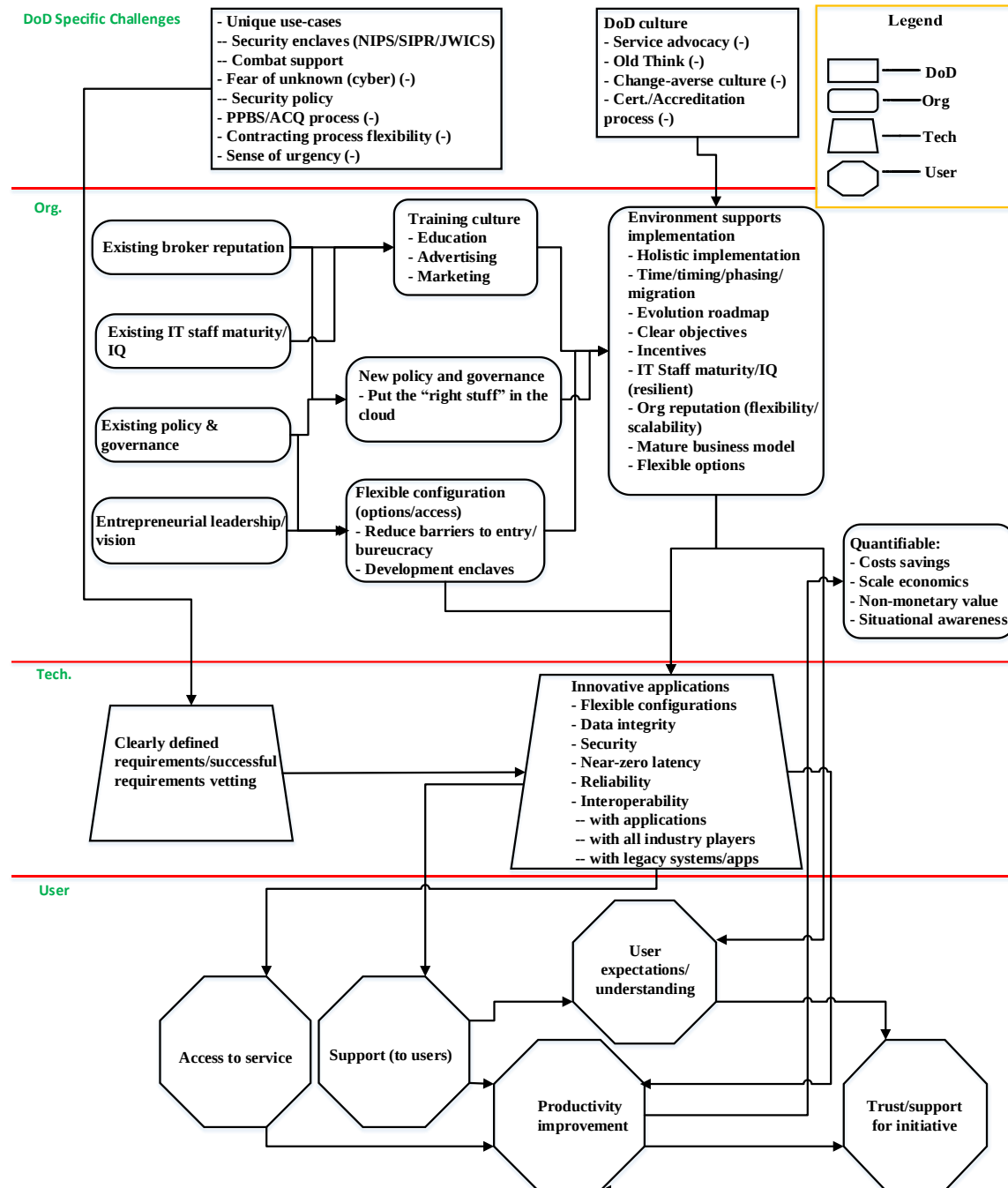
Figure 12. Process Model
