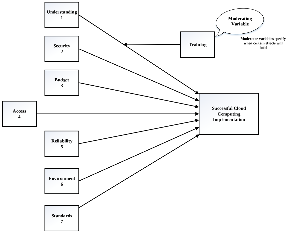
Figure 11. Variance Model
