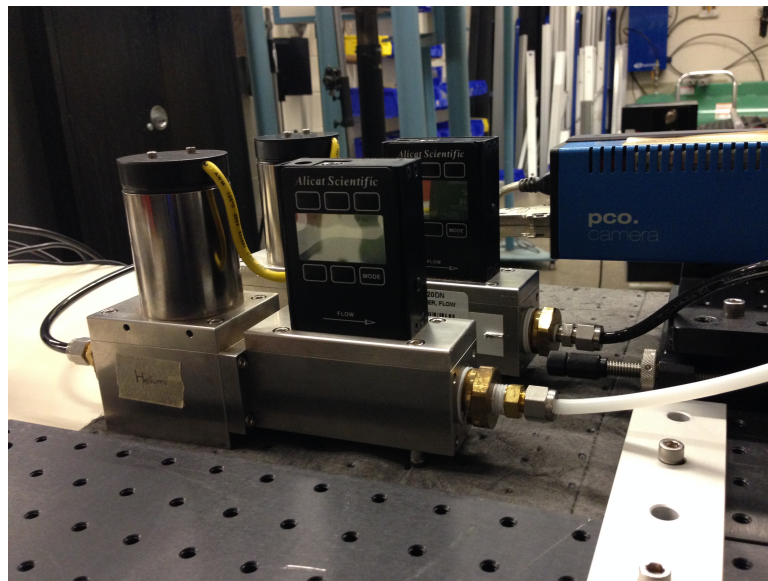
Figure 3.13: Alicat Scientific mass flow meters used for mixing gas and purge air
