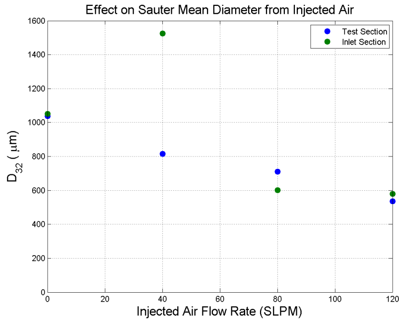
Figure 4.34: Particle statistics: Sauter mean diameter comparison between inlet and test sections for Mach 0.026
