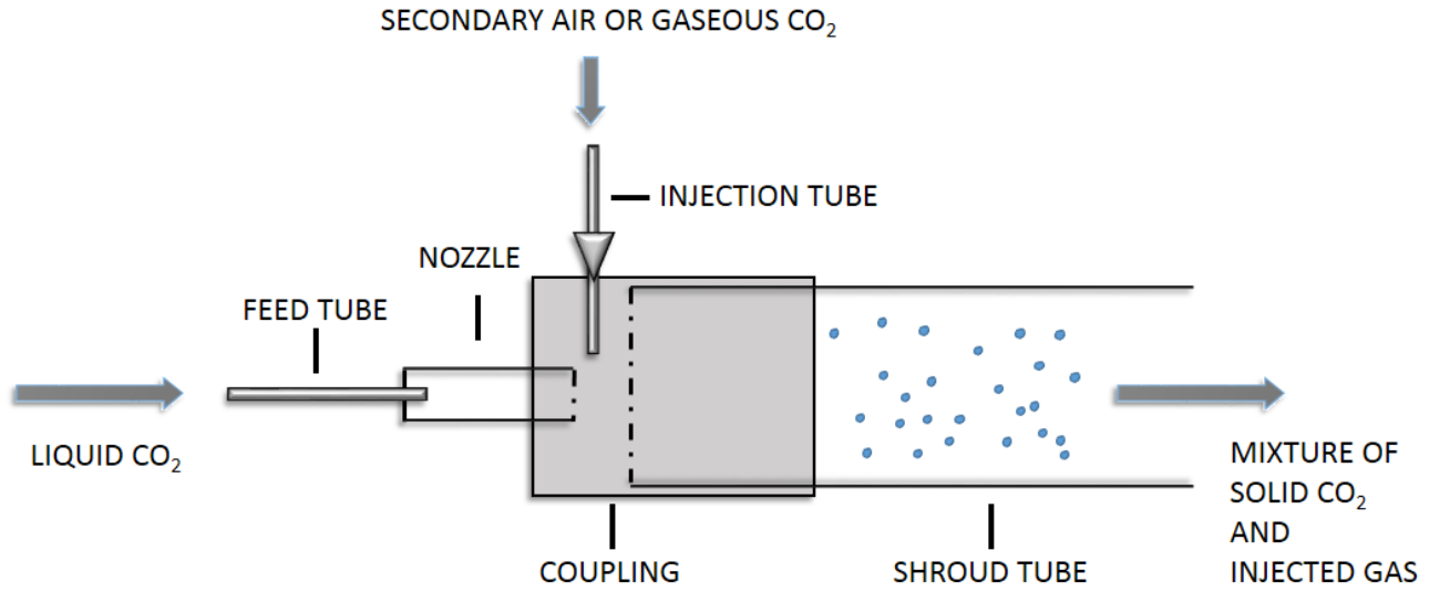
Figure 3.12: Schematic of secondary injection system with CO 2 injector
