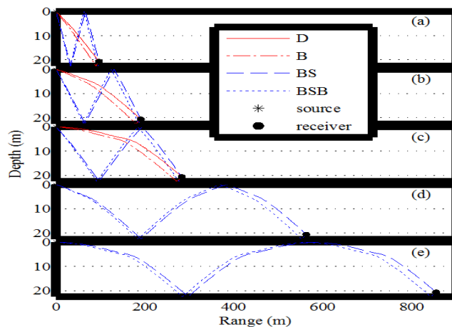
Figure 7: Ray trace using Bellhop. Only D, B, BS, and BSB eigenrays are shown. Note the culling of the D and B eigenrays as the range approaches 300 m. Panel (c) represents the maximum range of the D eigenray, which corresponds to a 0 degree ray launch angle. Likewise, panel (e) shows the maximum range of the BS eigenray.
