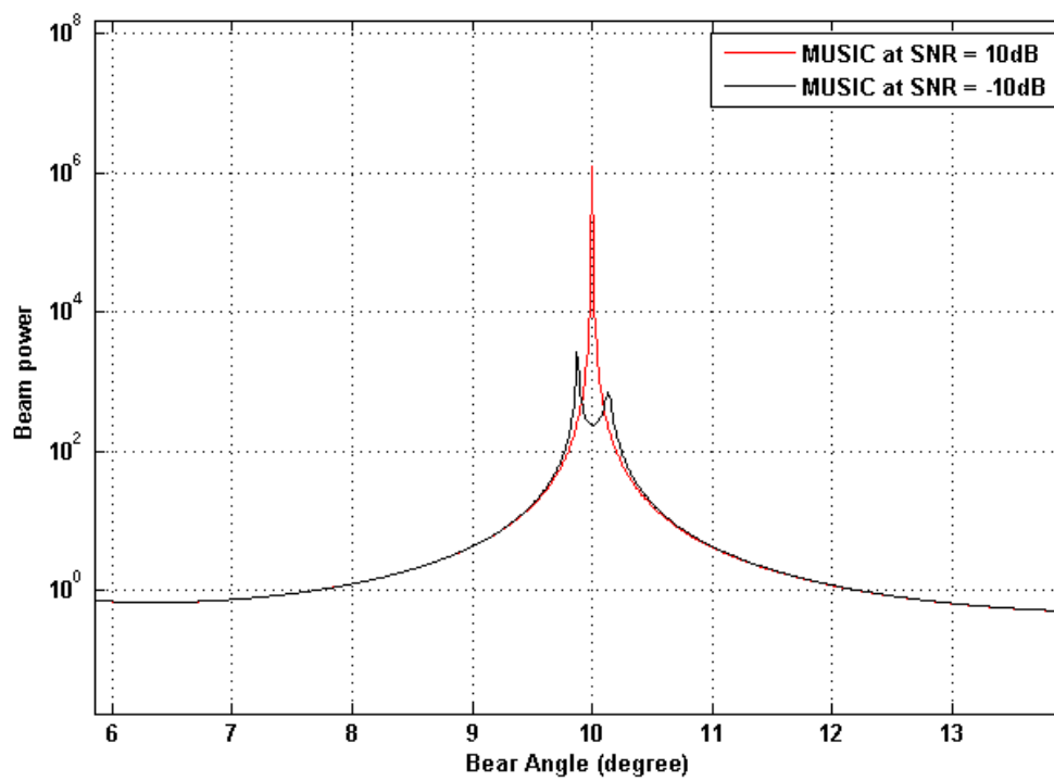
Figure 3.5: MUSIC at different SNR levels.
