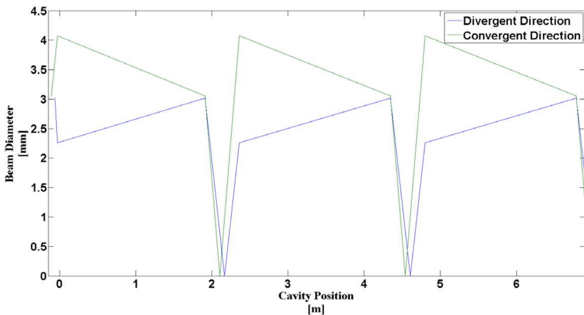
Figure 2. Plot of counterpropagating pulse beam diameter as a function of position within the 2.44 m cavity. Due to the asymmetric nature of the intracavity Keplerian telescope, the Keplerian focal points of the counterpropagating pulses, though not coincident in this plot, are indeed collocated spatially within the Keplerian lens set.
