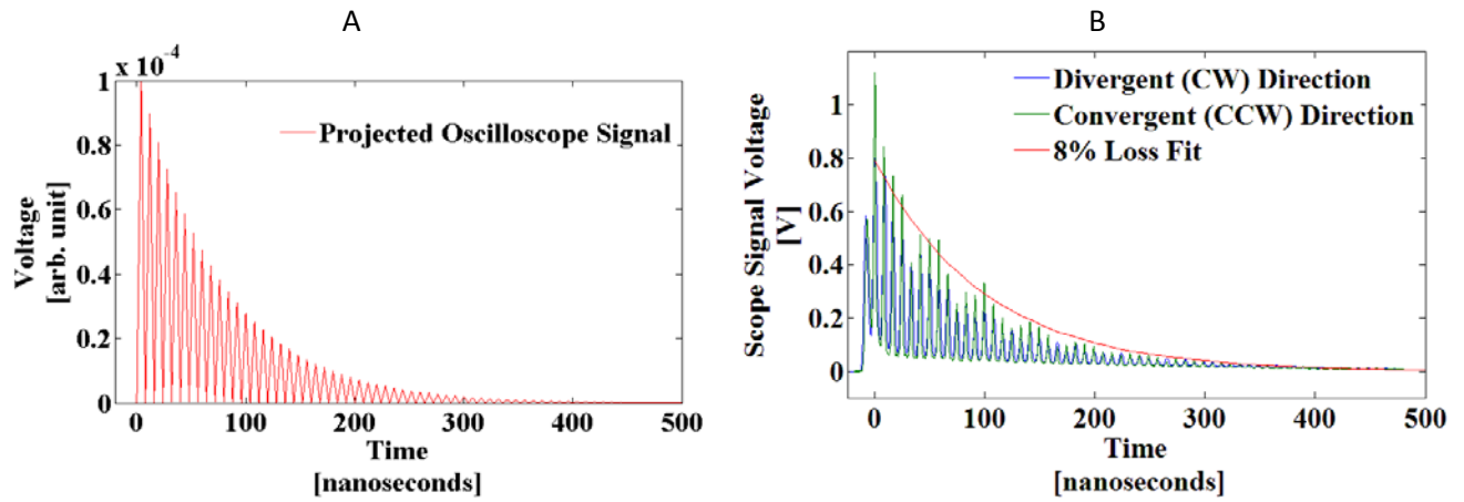
Figure 3.A.) Projected oscillogram based on an induced 10% round trip loss with a cavity length-dependent 8.1 ns round trip period. B.) Broadband 4 mJ Nd:YAG laser oscillogram of purposely induced cavity loss indicating cavity round trips and laser pulse temporal superposition in both the convergent and divergent cavity directions. Please note that the pulse at time t=0 is the initial s-polarized kick upon cavity pulse injection.
