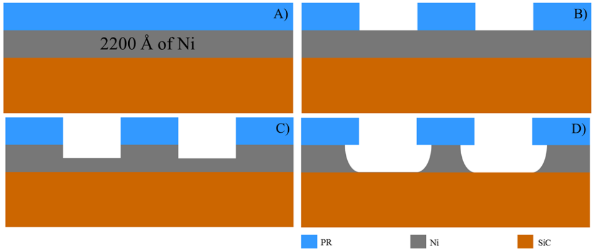
Figure 31 – The image above outlines the process of utilizing a 2200\ \text{\AA} thick Ni mask. The remaining Ni seen in D) is thick enough to allow sufficient time in the RIE to create SiC pillars \sim 7\ \mu\text{m} high.
