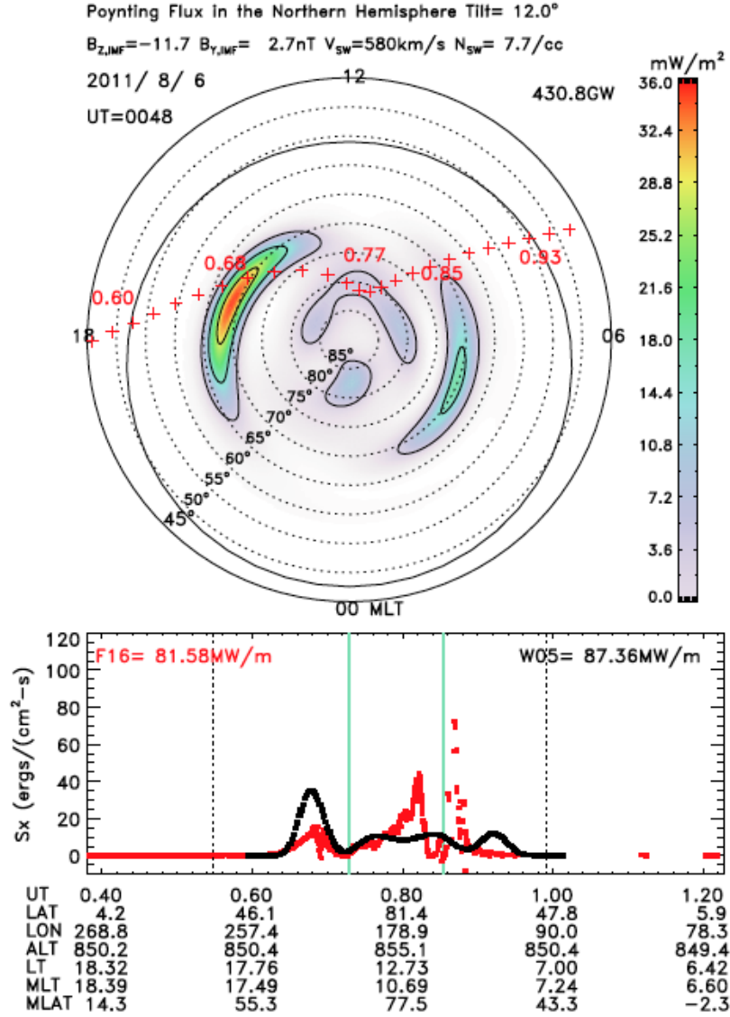
Figure 3. Top: spatial distribution of Poynting flux modeled by Weimer05 around 0050UT on August 6, 2011. The red crosses indicate the trajectory of F16. Bottom: comparison of Poynting fluxes along trajectory measured by F16 (red) and predicted by Weimer05 (black). The total Poynting fluxes integrated along trajectory are also shown, which is around 82 MW/m for F16, and 87 MW/m for Weimer05. The two vertical green lines indicate the convection reversal boundaries, and the two dotted lines indicate the magnetic latitude of 45 degrees.
