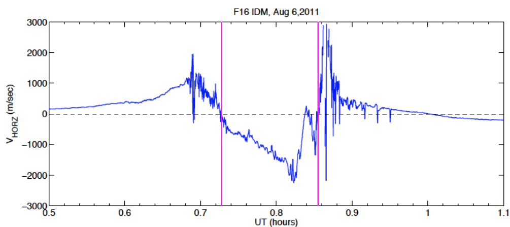
Figure 2. The horizontal component of Ion Drift Meter (IDM) data measured by DMSP F16 from 0030 UT to 0106 UT on August 6, 2011. The magenta vertical lines illustrate the convection reversal boundaries (CRBs).
