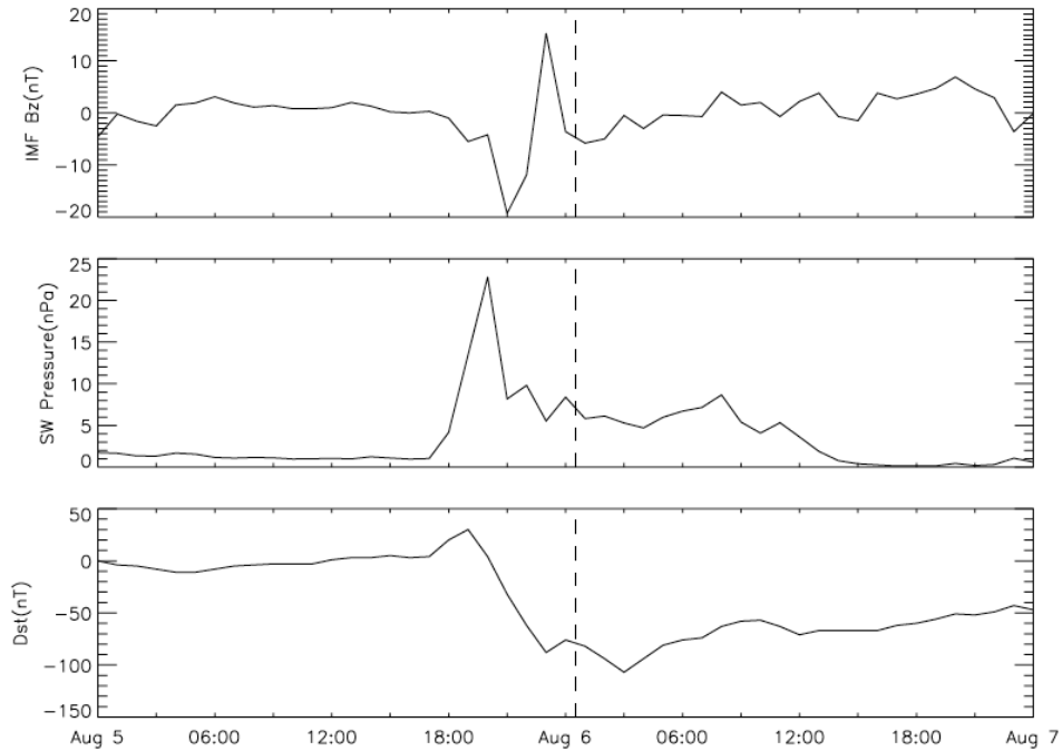
Figure 1. Temporal variations of the IMF Bz, the dynamic pressure of solar wind, and Dst index during a storm occurred on August 6, 2011. The dashed vertical lines indicate the start of DMSP measurements.
