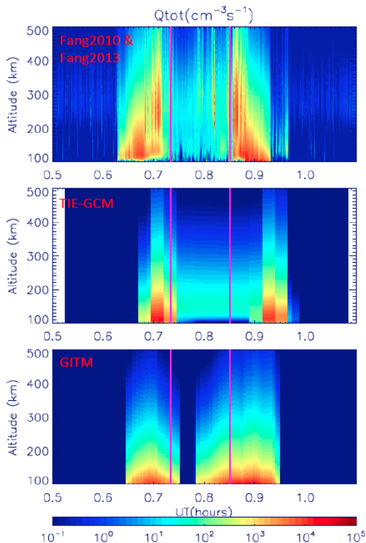
Figure 9. Comparison of total impact ionization rates calculated from (a) Fang2010 and Fang2013 parameterizations, (b) TIE-GCM and (c) GITM along the F16 trajectory for the August 6, 2011 storm.
