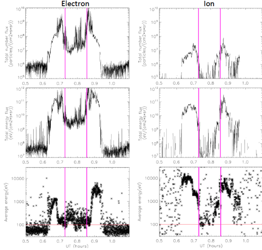
Figure 5. First row: the total number flux of electrons (left) and ions (right) measured by DMSP F16 satellite. The two vertical magenta lines indicate the convection reversal boundaries. Second row: the total energy flux of electrons (left) and ions (right). Third row: the mean energy of electrons (left) and ions (right) obtained through dividing the total energy flux by the total number flux. The red line illustrates the 100 eV particle energy.
