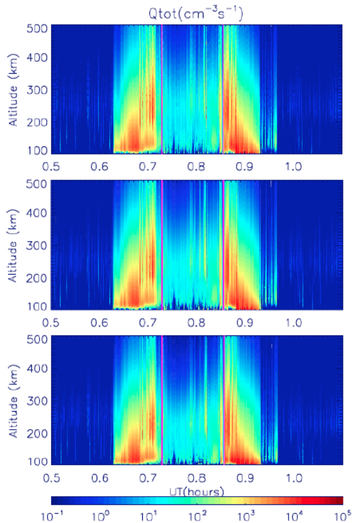
Figure 7. Altitudinal variation of total particle impact ionization rate calculated from Fang2010 (electrons) and Fang2013 (ions) parameterizations along the F16 trajectory using thermosphere simulated by the NRLMSISE-00 model (first row), TIE-GCM (second row) and GITM (third row) in Figure 6. The two vertical magenta lines indicate the convection reversal boundaries.
