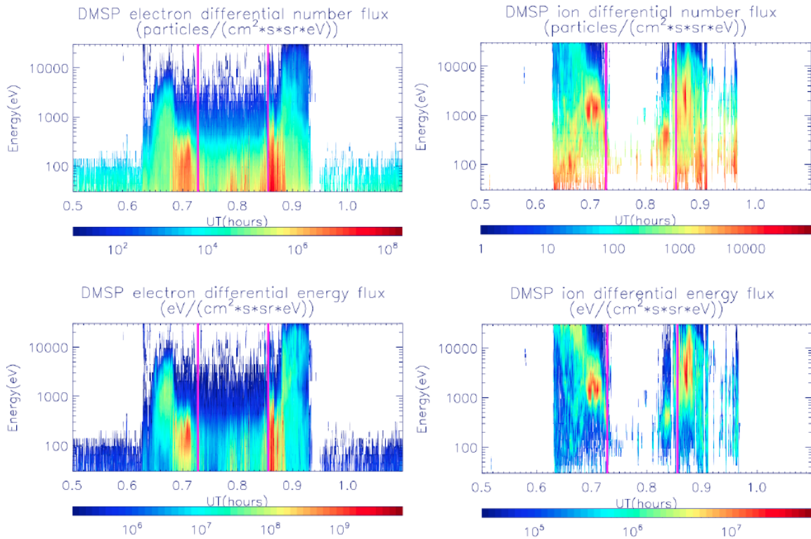
Figure 4. Left column: differential number and energy fluxes of electrons measured by DMSP F16 satellite over the northern hemisphere on August 6, 2011. Right column: differential number and energy fluxes of ions.
