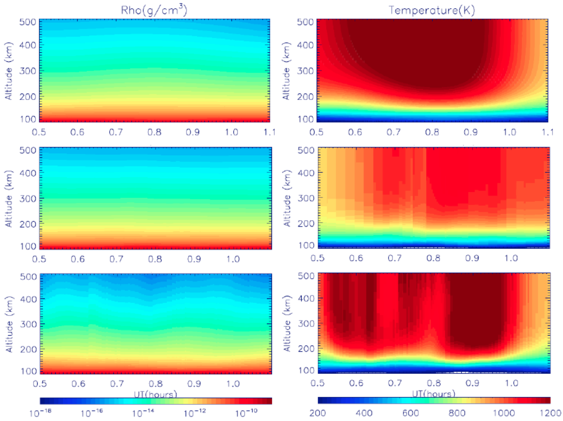
Figure 6. Altitudinal variation of neutral density and temperature along the F16 trajectory from 0030UT to 0106UT simulated by the NRLMSISE-00 model (first row), TIE-GCM (second row) and GITM (third row).
