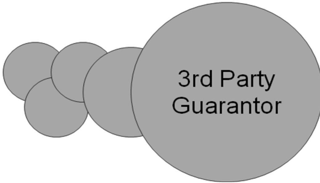
Figure 4. Third-party guarantor
