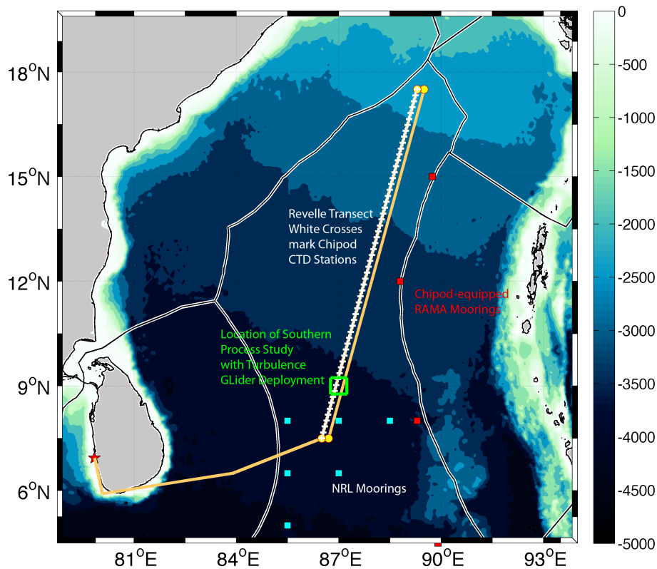
Figure 1: Map of study region. NRL mooring locations (white squares), RAMA mooring locations (red squares), survey transect path, and process study location (green box) are indicated. Tentative \chi pod CTD stations are shown with white crosses.
