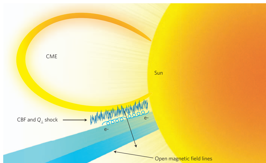
Figure 1 | Coronal mass ejection. The CME observed on 22 September 2011 drove a coronal bright front (CBF) and quasiperpendicular ( Q_{\perp} ) shock southwards along the limb of the Sun. Shock-accelerated electrons escape to interplanetary space along open field lines.
