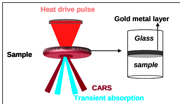
Figure 1. Schematic diagram for flash heating experiment.
