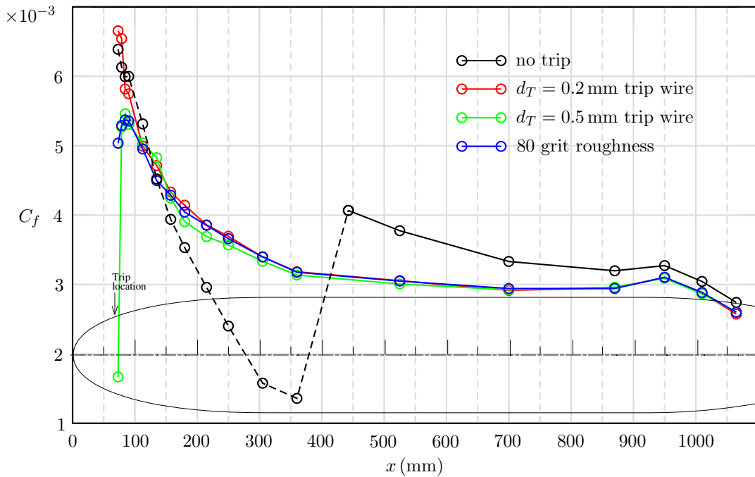
Figure 16: Comparison of trip devices for U_\infty = 40 m/s. For un-tripped data dashed curve indicates a measurement in laminar/transiting boundary layer. Model profile and trip location also shown.
