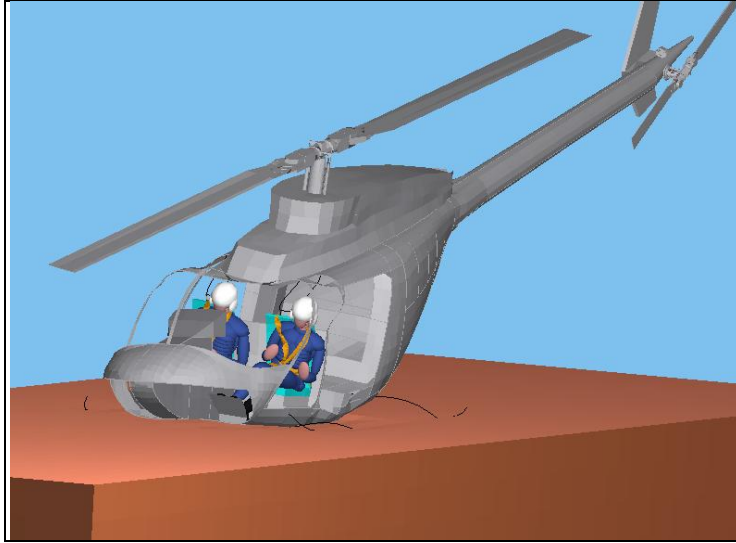
Figure 15. Helicopter model impacting vertically at 10° (nose-down) pitch and 10° (port) roll.
