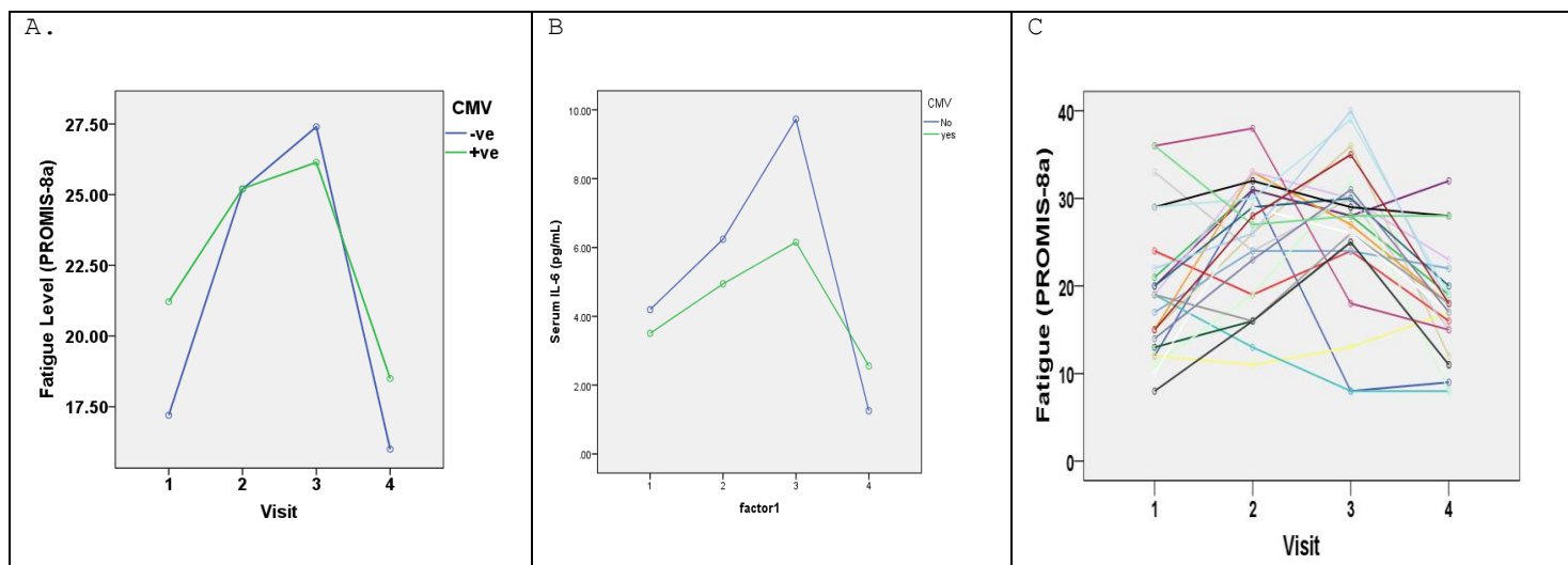
Figure 3: Fatigue and Inflammation during chemotherapy for breast cancer: results of the IDEA award-funded study. A: Self-reported fatigue level at each of the 4 study visits. The mean values for CMV seropositive participants (n=14) and CMV seronegative participants (n=10) are shown. Fatigue increased sequentially during chemotherapy, as expected, but did not differ by CMV status. B: Mean serum IL-6 levels for CMV+ and CMV- participants over the course of the study. IL-6 levels increased over the course of the study and correlated with fatigue, but were not significantly affected by CMV. C: The fatigue levels are graphed separately for each individual, revealing different patterns in fatigue trajectory among the study participants.
