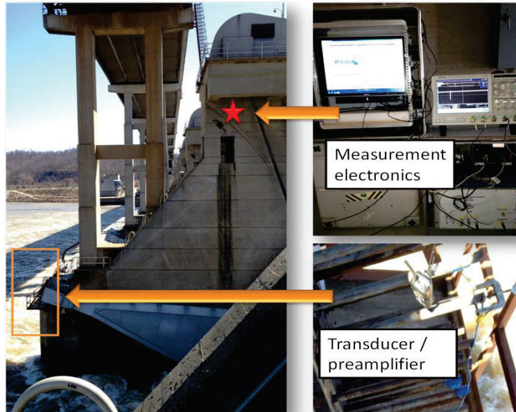
Figure 5. Location of testing equipment at Greenup Lock and Dam.
