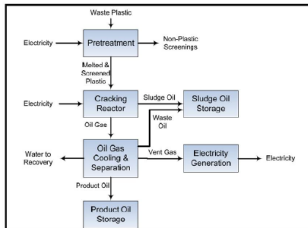
Figure 2: Envion Pyrolysis Process Flow Diagram (Source: www.envion.com )
