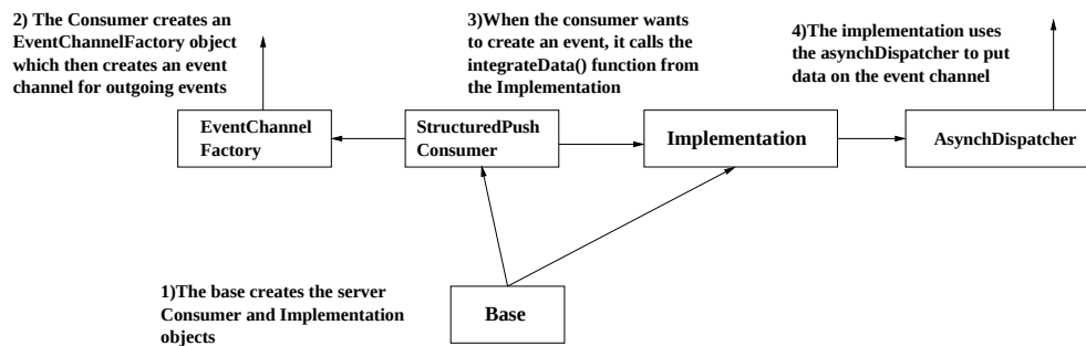
Figure 11: ExampleC Structure
