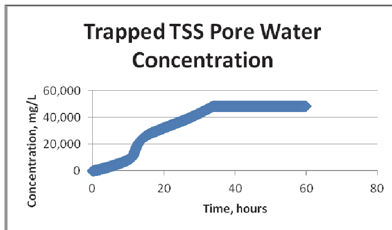
Figure 7. TSS pore water concentration trapped in filter 1 versus time for single storm event.
