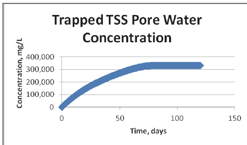
Figure 14. TSS pore water concentration trapped in filter 1 versus time for steady continuous rainfall.
