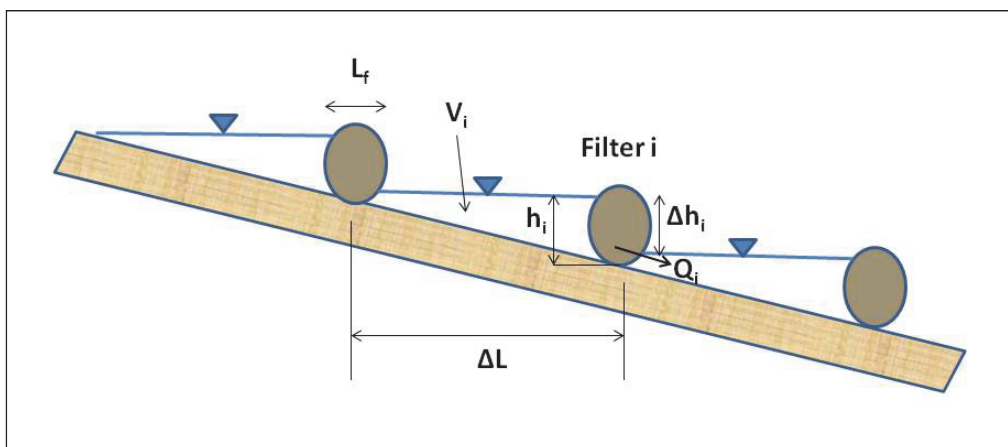
Figure 3. Profile view for schematic of a cascade of filters.
