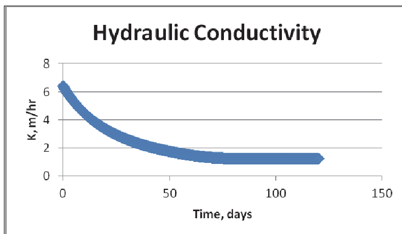
Figure 16. Hydraulic conductivity versus time for filter 1 and steady continuous rainfall.
