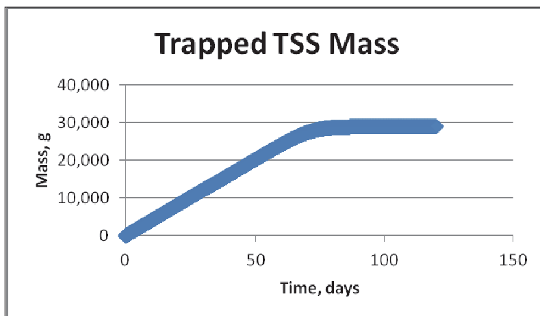
Figure 17. TSS mass trapped within filter 1 for a steady continuous rainfall.
