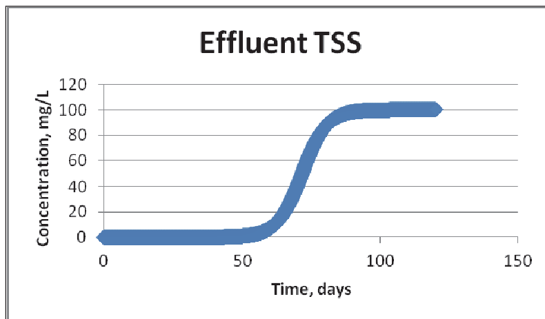
Figure 15. TSS effluent concentration versus time for filter 1 and steady continuous rainfall.
