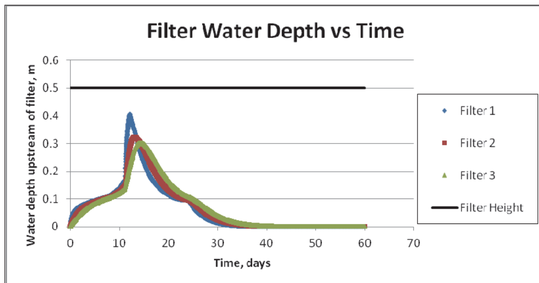
Figure 4. Filter approach depth versus time for each filter compared to the filter height for a single storm event.
