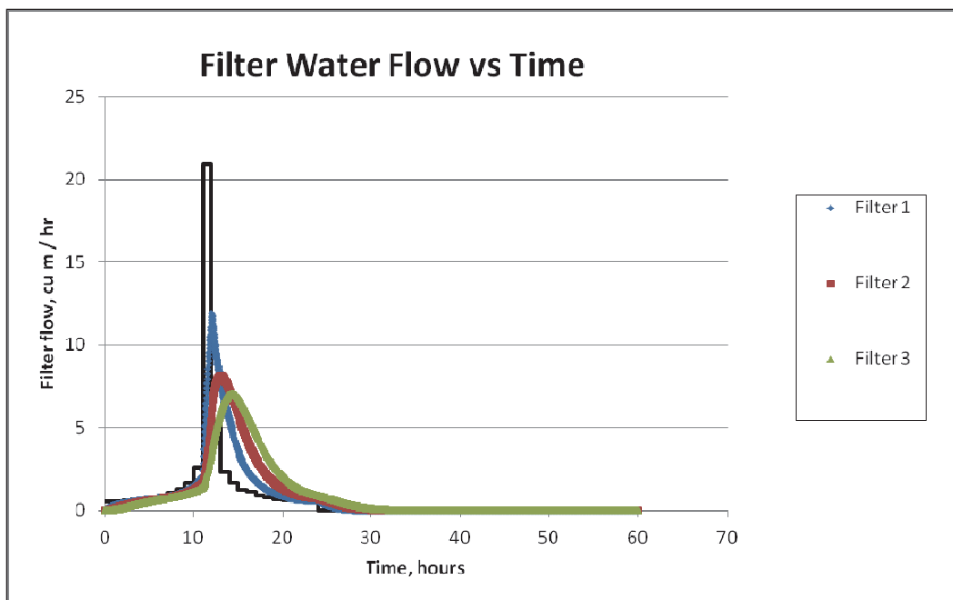
Figure 5. Filter flow rate (cubic meters per hour) versus time for each filter compared to the AOI runoff flow rate for a single storm event.
