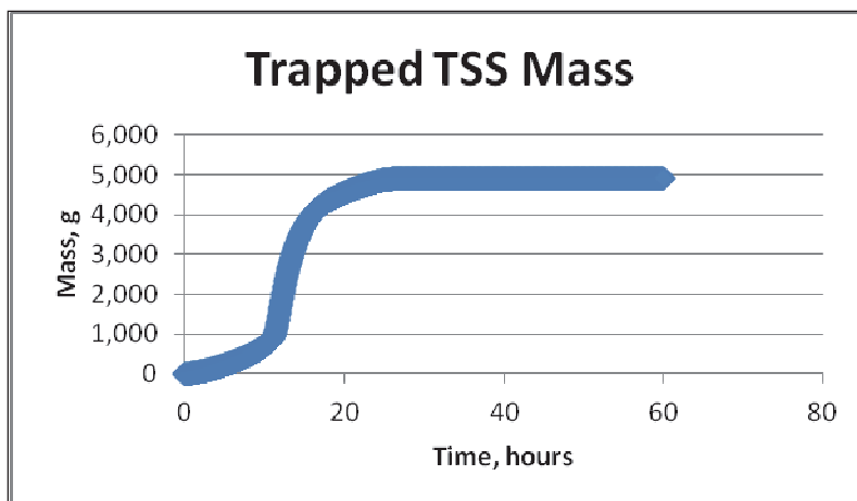
Figure 10. Trapped TSS mass versus time within filter 1 for a single storm event.
