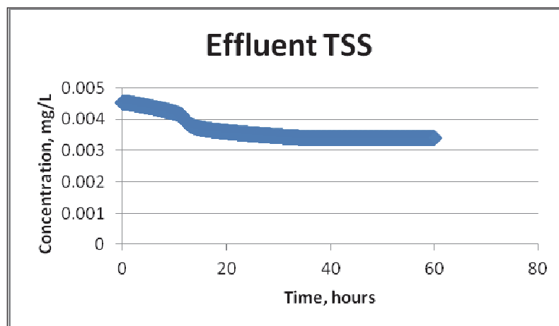
Figure 8. TSS effluent concentration versus time for filter 1 and single storm event.
