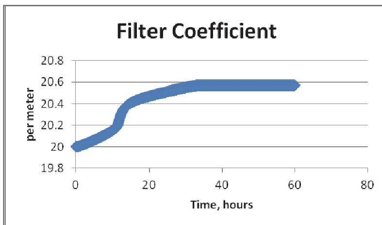
Figure 6. Filter removal coefficient versus time for filter 1 and single storm event.
