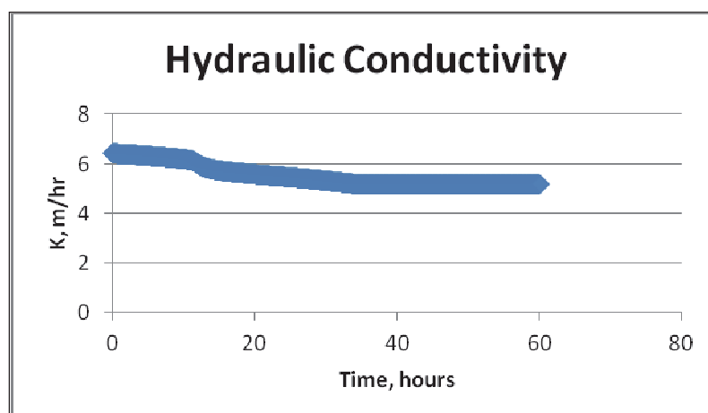
Figure 9. Hydraulic conductivity versus time for filter 1 and single storm event.
