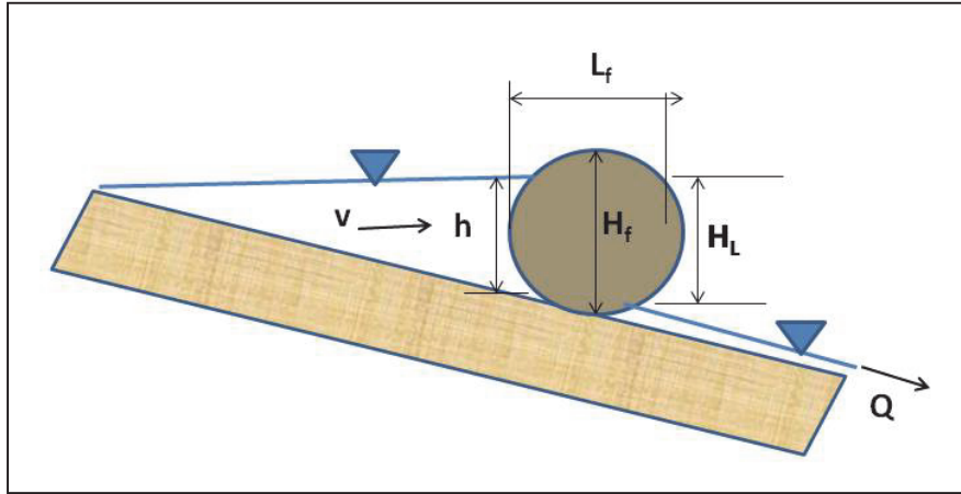
Figure 2. Flow schematic of filter tube.
