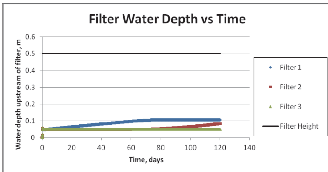
Figure 11. Filter approach depth versus time for each filter compared to the filter height for continuous steady rainfall.
