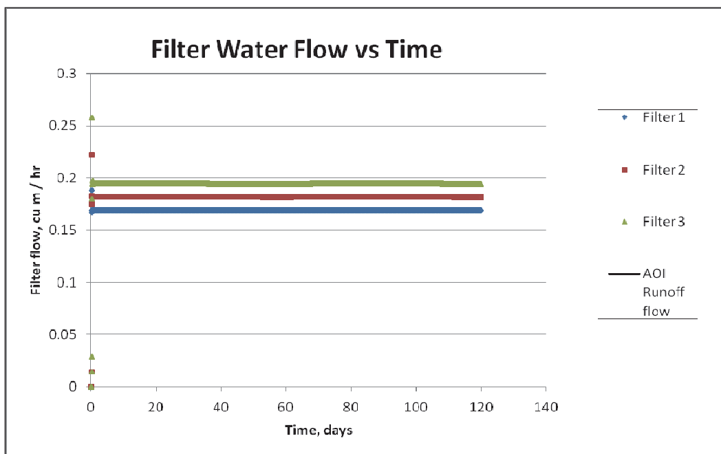
Figure 12. Filter flow rate versus time for each filter compared to the AOI runoff flow rate for continuous steady rainfall.
