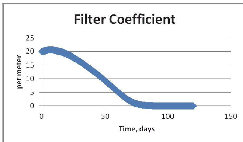
Figure 13. Filter removal coefficient versus time for filter 1 and steady continuous rainfall.
