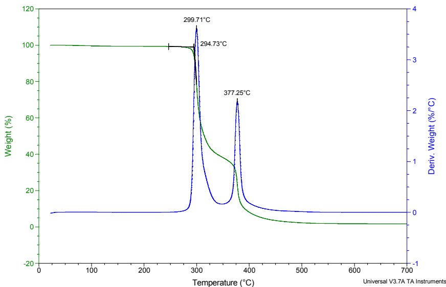
Figure 1. Thermogram of Texin 950D showing plots of %wt versus T and d(\text{wt}\%)/dT versus T.
