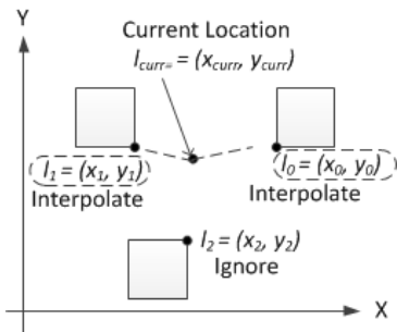
Figure 4: Linear interpolation
