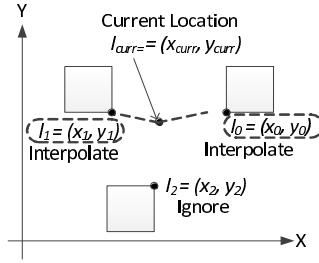
Fig. 7 Linear interpolation
