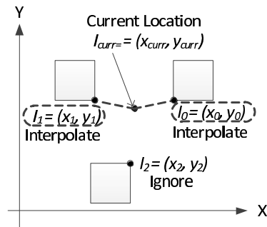
Figure 4: Linear interpolation
