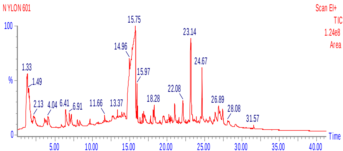
Figure 40. Pyrogram of a sample of Nylon 6.
