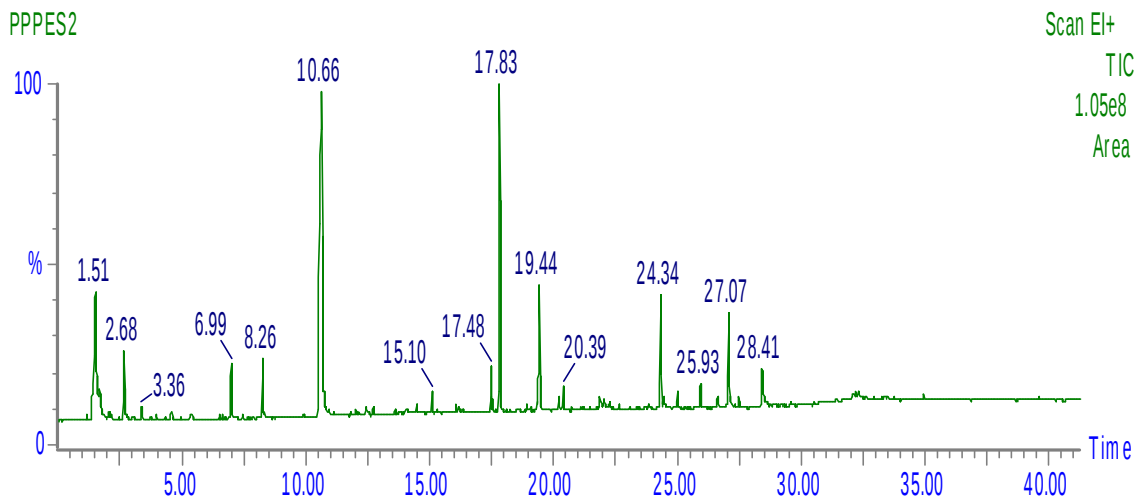
Figure 24. Pyrogram of a sample of poly(p-phenylene ether sulfone).
