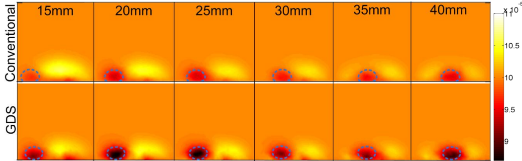
Fig.3 Piece-wise simulation results with varied target longitudinal position variation in sagittal-middle plane of the imaging geometry.
