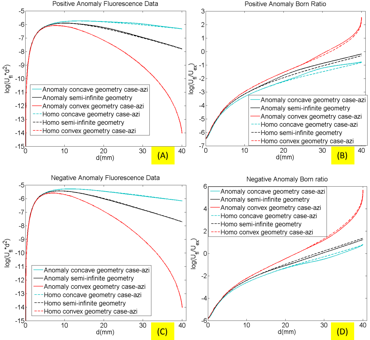
Figure 6. The comparisons of the change of fluorescent measurement due to an anomaly with fluorescence contrast in concave , convex and semi-infinite geometry in case-azi. (A) The change in fluorescence data due to a positive contrast anomaly. (B) The change in Born ratio due to a positive contrast anomaly. (C) The change in fluorescence data due to a negative contrast anomaly. (D) The change in Born ratio due to a negative contrast anomaly. It is indicated that the fluorescent measurement is less sensitive to negative contrast anomaly than positive contrast anomaly and Born ratio is more sensitive to the anomaly inclusion than only the fluorescent data.
