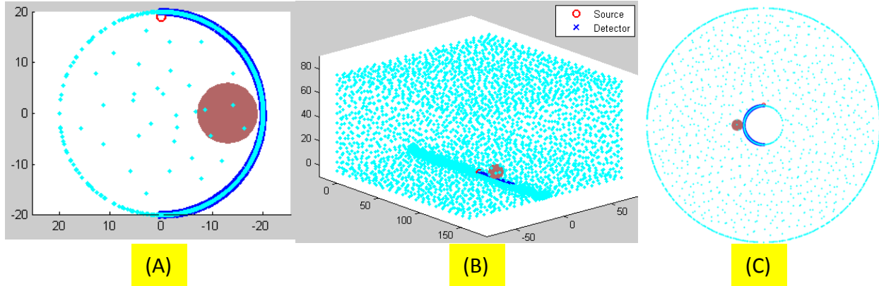
Figure 4. FEM imaging volume for case-azi. Detectors are aligned along the azimuth plane on the applicator's interface. (A) concave geometry, (B) semi-infinite geometry, (C) convex geometry.
