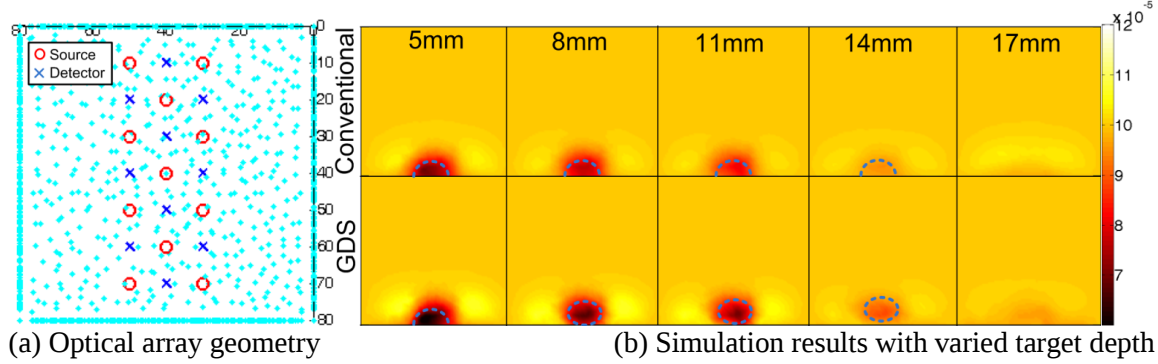
Fig.2 Optical array geometry used in piece-wise simulation study. The numbers at the top of each column in (b) indicated the actual center-to-bottom depths of the targets
