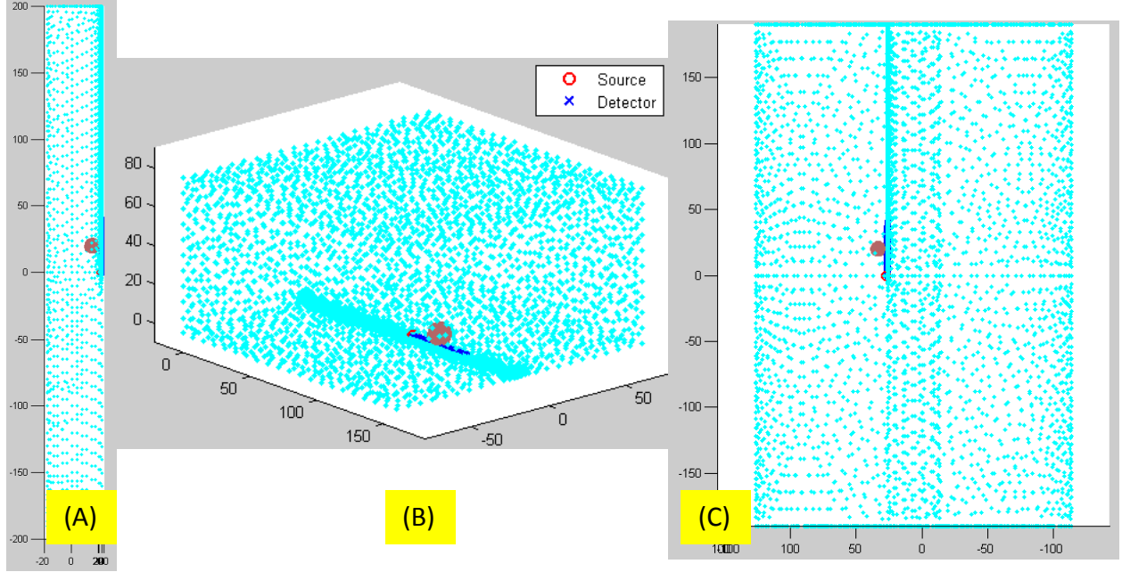
Figure 5. FEM imaging volume for case-longi. Detectors are aligned longitudinally with same azimuth angle on the applicator's interface. (A) concave geometry, (B) semi-infinite geometry, (C) convex geometry.
