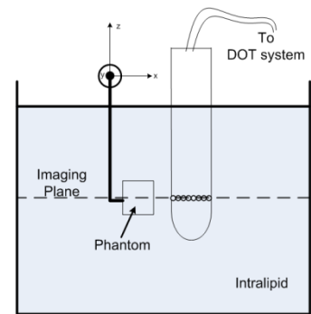
Fig 6 Experiment setup
