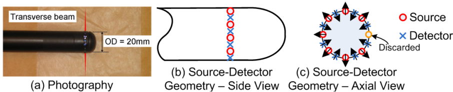
(a) Photography (b) Source-Detector Geometry - Side View (c) Source-Detector Geometry - Axial View Fig.2 A circular endoscopic imaging geometry
