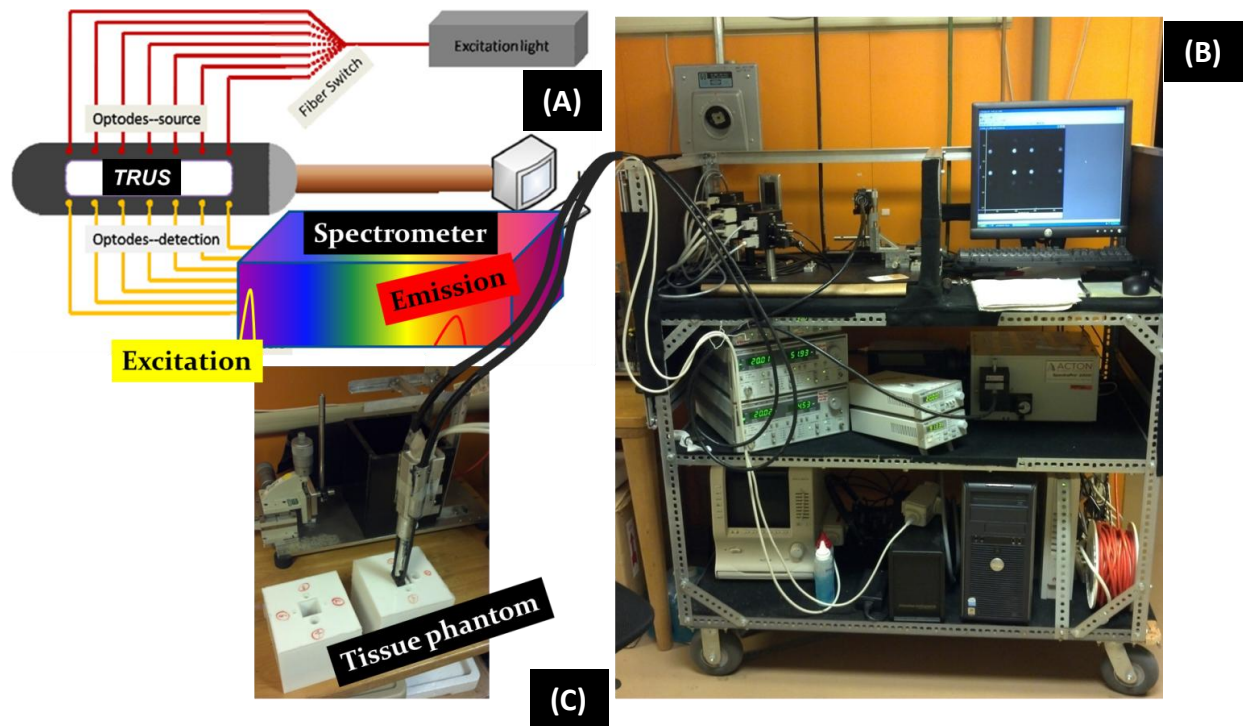
Figure 8. TRUS-coupled FDOT system. (A) System configuration. (B) The photograph of the system. (C) The applicator placed in a tissue phantom for positive-contrast test.
