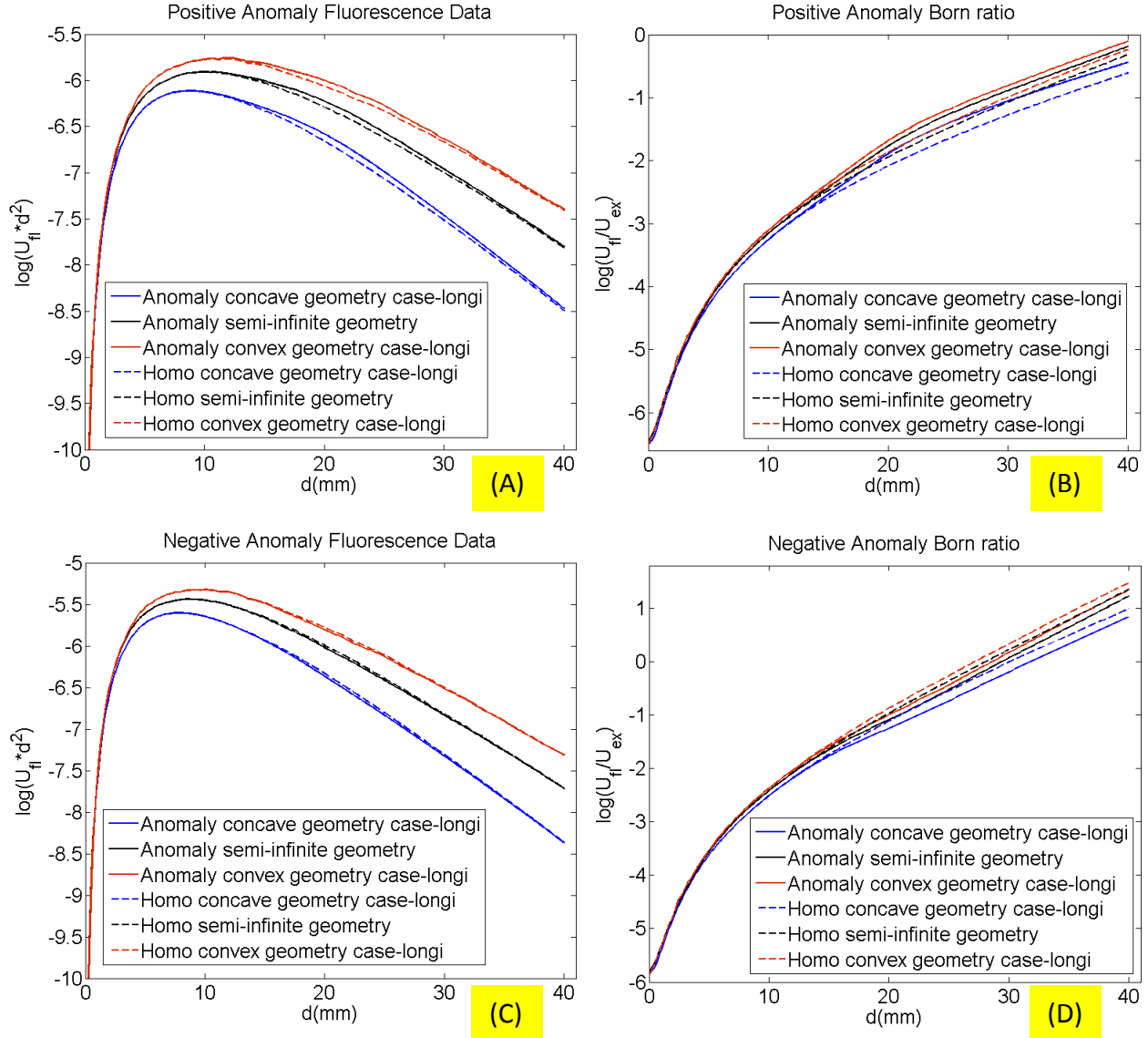
Figure 7. The comparisons of the change of fluorescent measurement due to an anomaly with fluorescence contrast in concave , convex and semi-infinite geometry in case-longi. (A) The change in fluorescence data due to a positive contrast anomaly. (B) The change in Born ratio due to a positive contrast anomaly. (C) The change in fluorescence data due to a negative contrast anomaly. (D) The change in Born ratio due to a negative contrast anomaly. It is indicated that the fluorescent measurement is less sensitive to negative contrast anomaly than positive contrast anomaly and Born ratio is more sensitive to the anomaly inclusion than only the fluorescent data.
