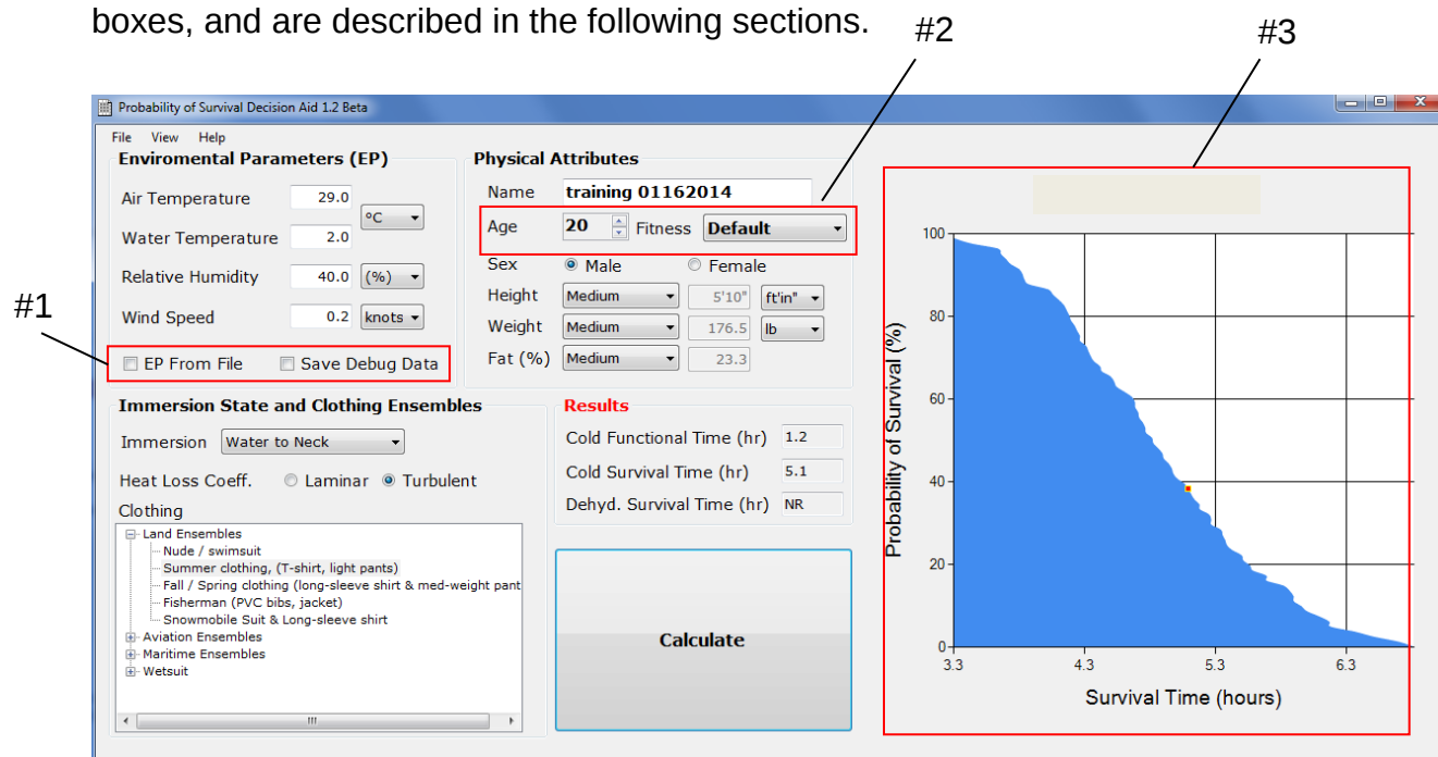
Figure 1. Probability of Survival Decision Aid (PSDA v1.2 beta) interface showing improvement #1, #2 and #3
