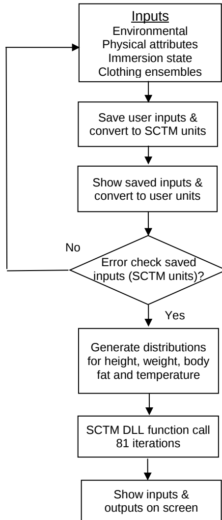
Figure 3. Graphic User Interface (GUI) Flowchart
