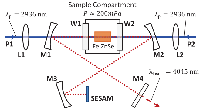
Fig. 1. A schematic view of the Fe:ZnSe laser design. All optics are made of \text{CaF}_2 and AR-coated at 2936 nm unless otherwise noted.
