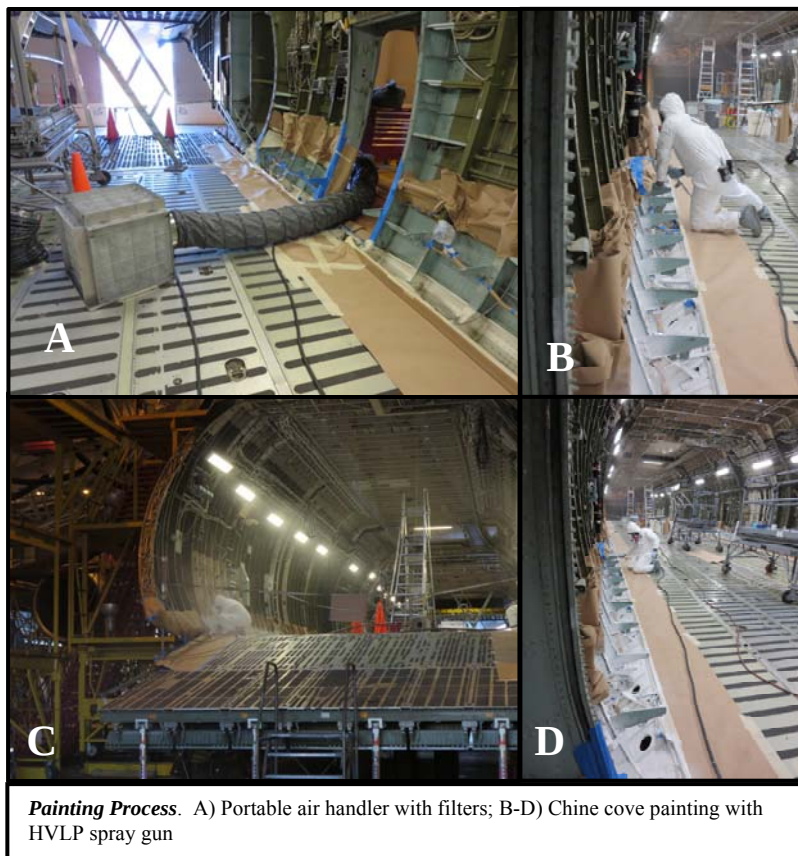
Figure 10. Painting Process
