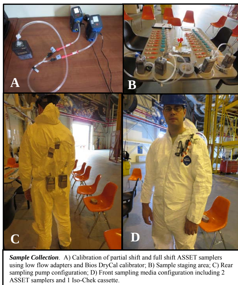
Figure 9. Sample Collection
