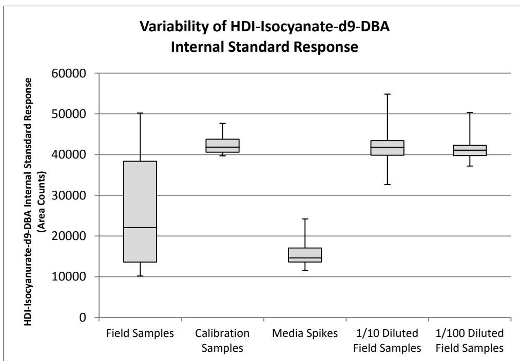
Figure 4. Variability of HDI-Isocyanate-d9-DBA Internal Standard Response
