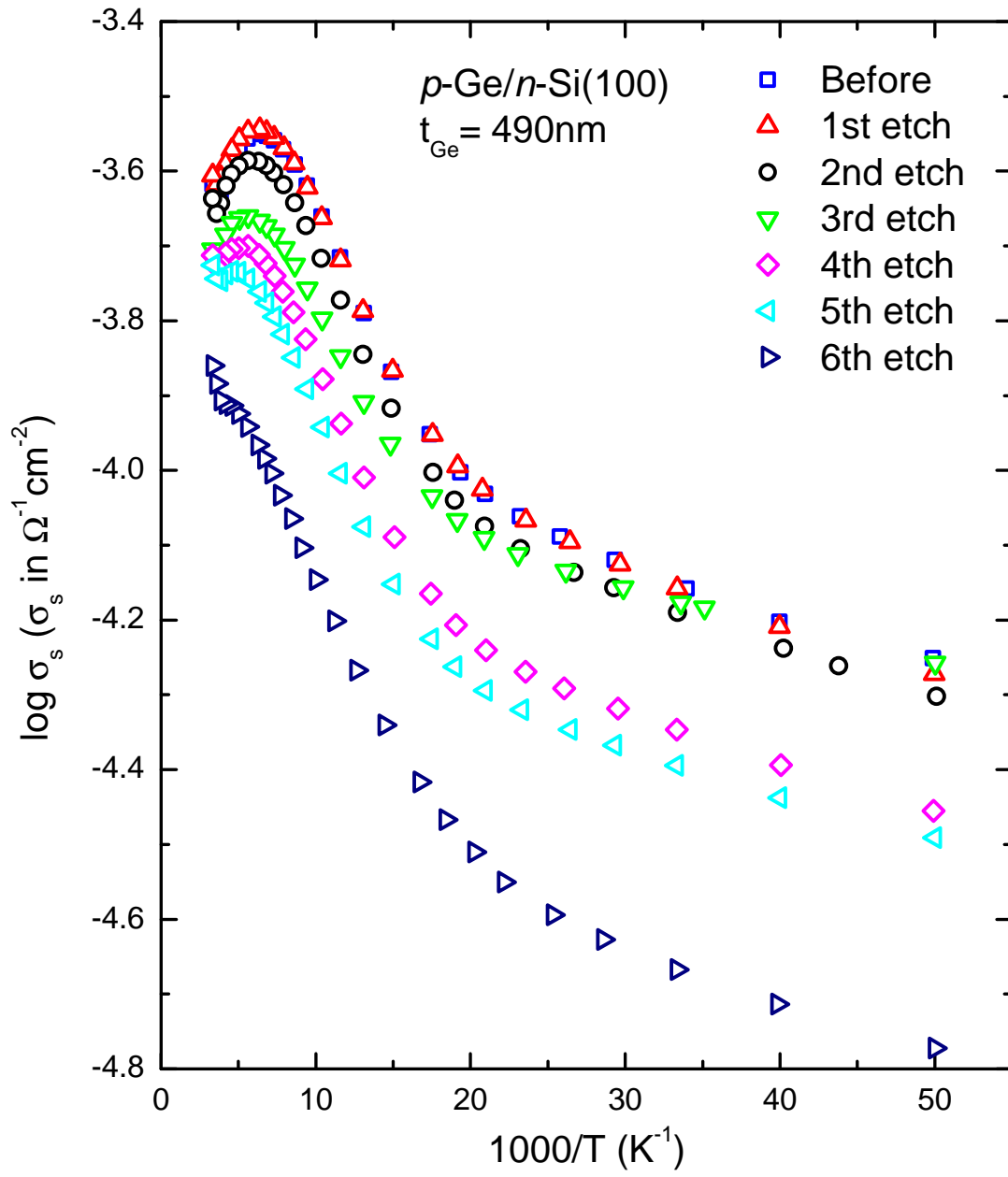
Figure 33. Log conductivity plotted as a function of inverse temperature for the p\text{-Ge}/n\text{-Si} sample for all etches.
