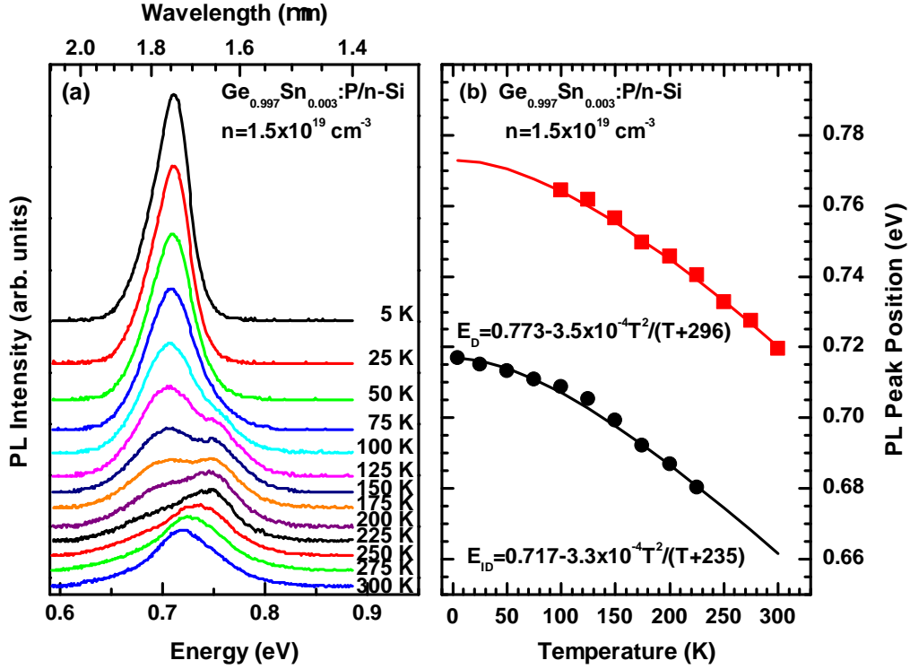
Figure 5. (a) Temperature-dependent PL spectra of the P-doped n - \text{Ge}_{0.997}\text{Sn}_{0.003} grown on n -Si substrate. (b) Direct ( E_D ; red squares) and indirect ( E_{ID} ; black circles) bandgap related PL peak energies plotted as a function of temperature from 5 to 300 K. The red and black fitting curves are the calculated direct ( E_D ) and indirect ( E_{ID} ) bandgap related energies, respectively, plotted as a function of temperature using Varshni equation.
