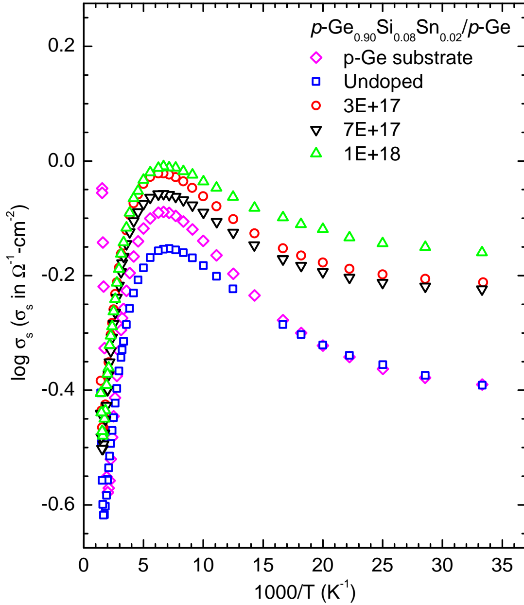
Figure 40. Log conductivity plotted as a function of inverse temperature for undoped and p -type doped \text{Ge}_{0.90}\text{Si}_{0.08}\text{Sn}_{0.02}/p\text{-Ge} samples along with the p -Ge substrate.
