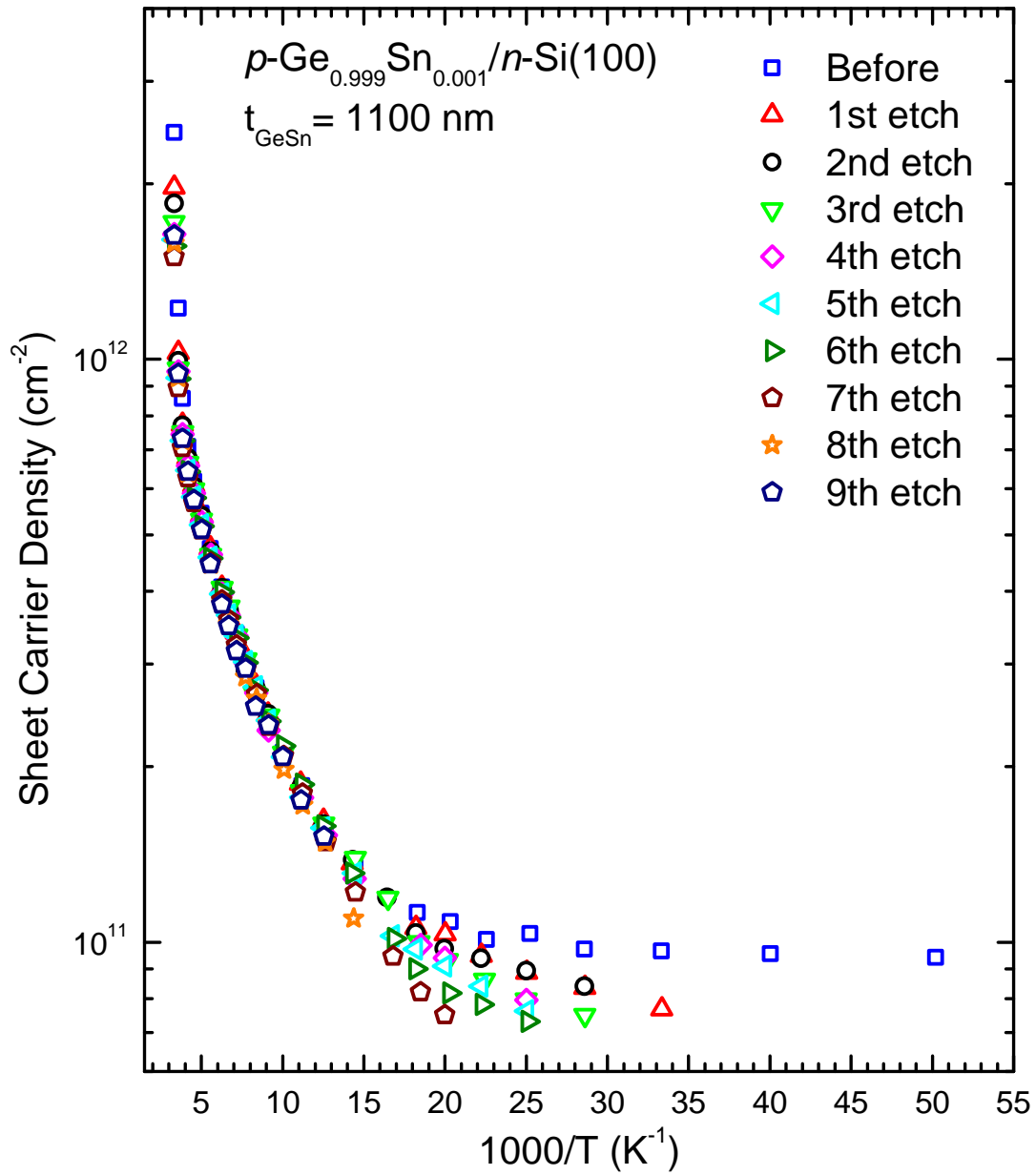
Figure 24. Sheet carrier concentration plotted as a function of inverse temperature for the p\text{-Ge}_{0.999}\text{Sn}_{0.001}/n\text{-Si} sample for all etches.
