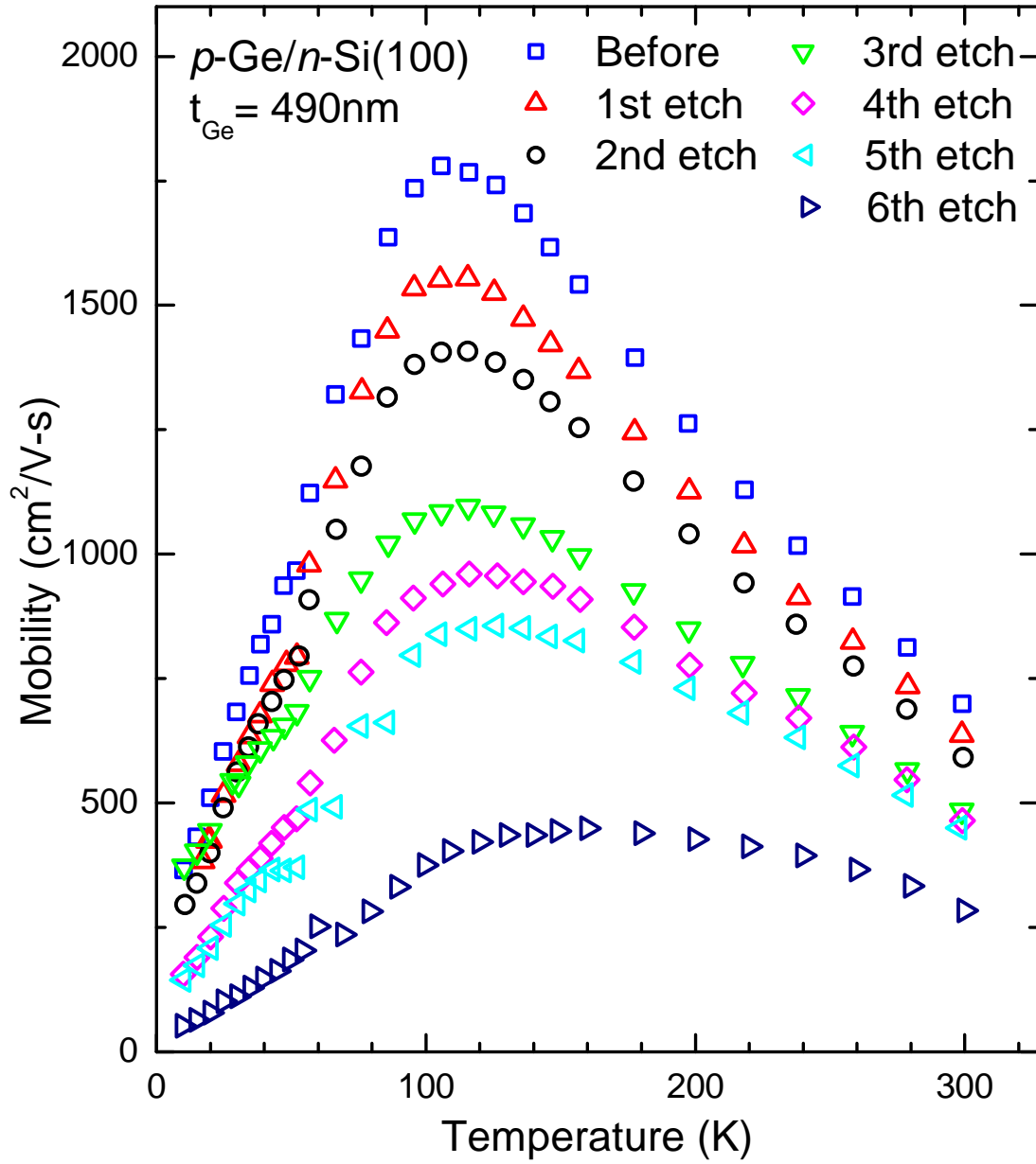
Figure 32. Carrier mobility plotted as a function of temperature for the p\text{-Ge}/n\text{-Si} sample for all etches.
